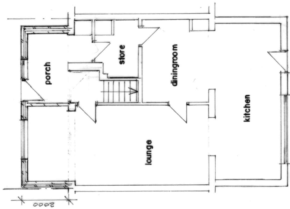
GROUND FLOOR PLAN (PROPOSED)
