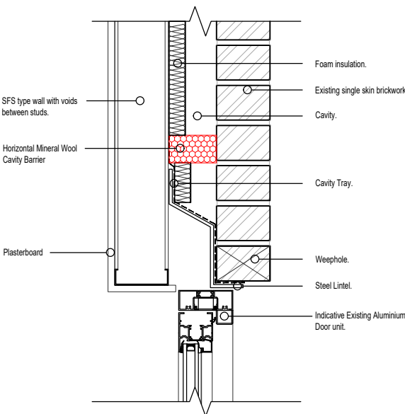
EXISTING - Typical Door Head - Brick - Scale 1:10
