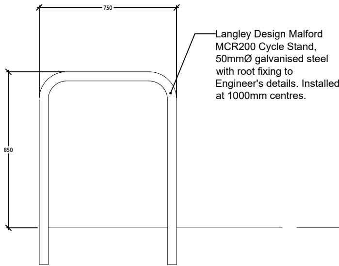
C5 Cycle Stands - Section detail 1:20
