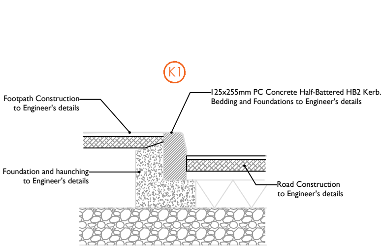
C1 Standard Kerb K1 - Section detail 1:20
