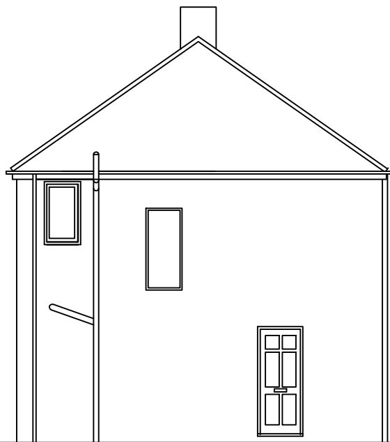
SIDE ELEVATION (facing No 33)
