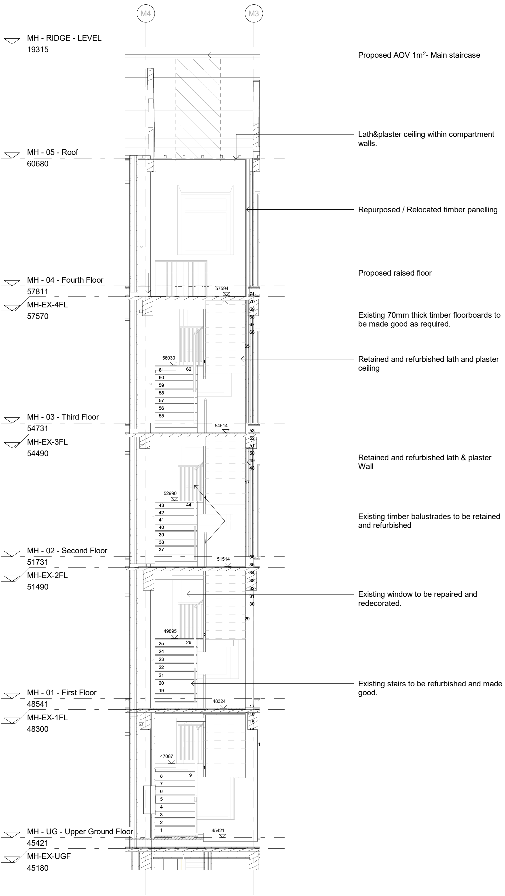
B | MAIN STAIR CORE SECTION 1 : 50
