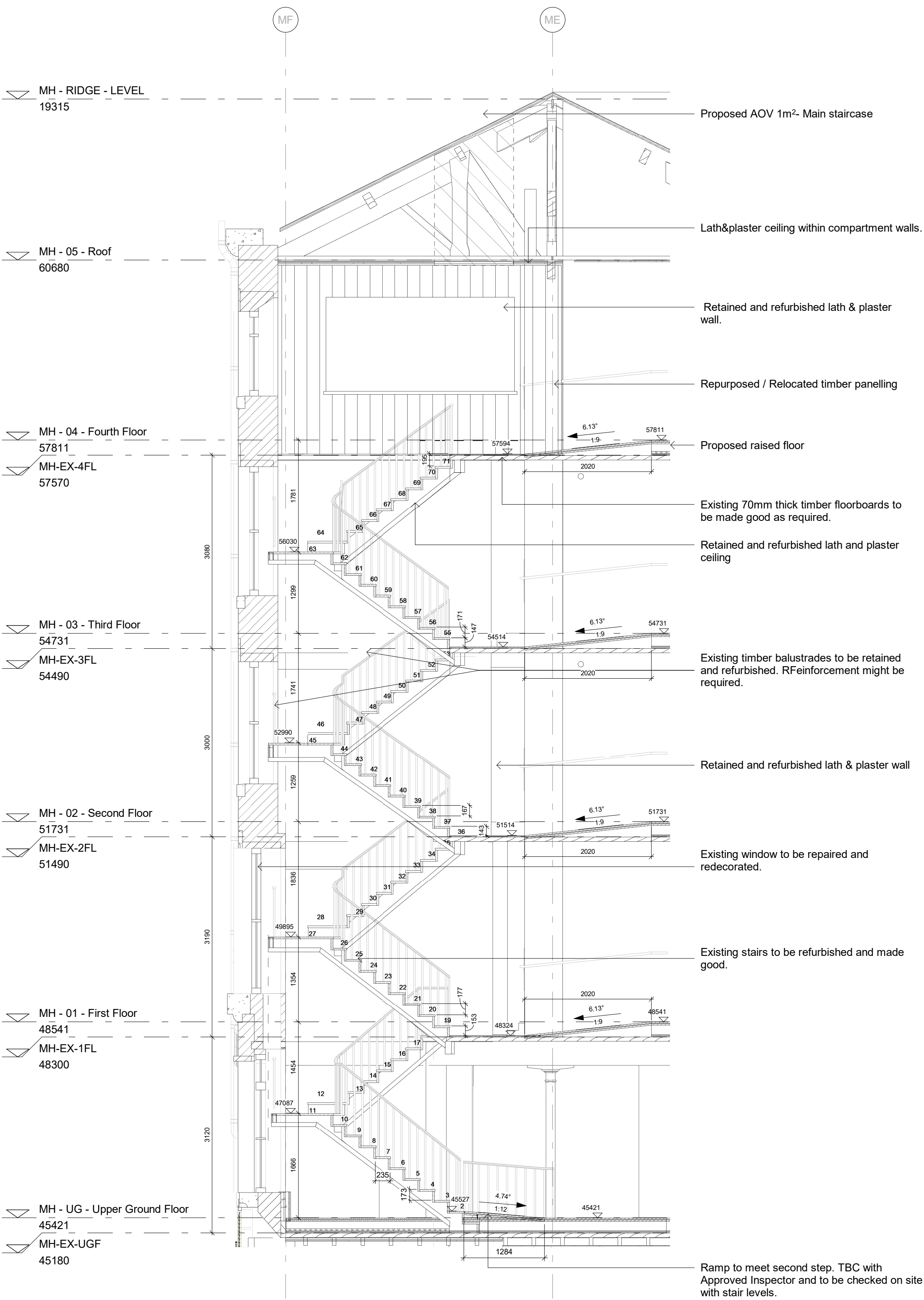
A | MAIN STAIR CORE SECTION 1 : 50
