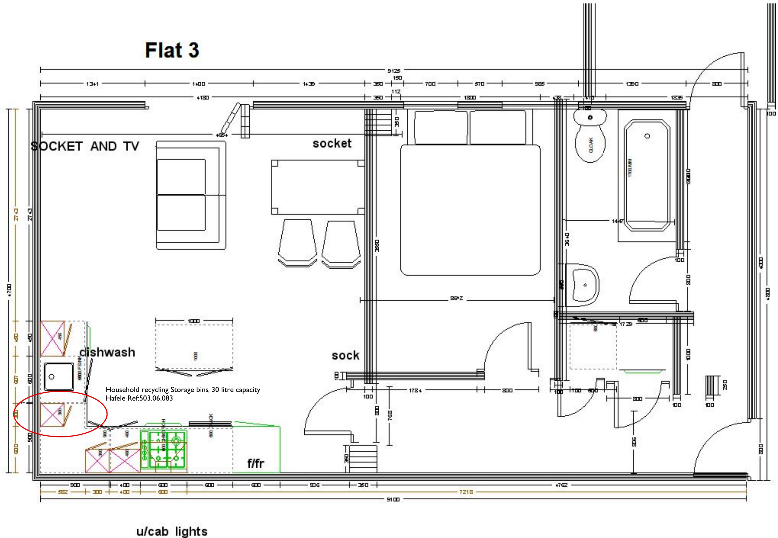
Apartment 03, 24 Whalley Range - Proposed Kitchen Layout
