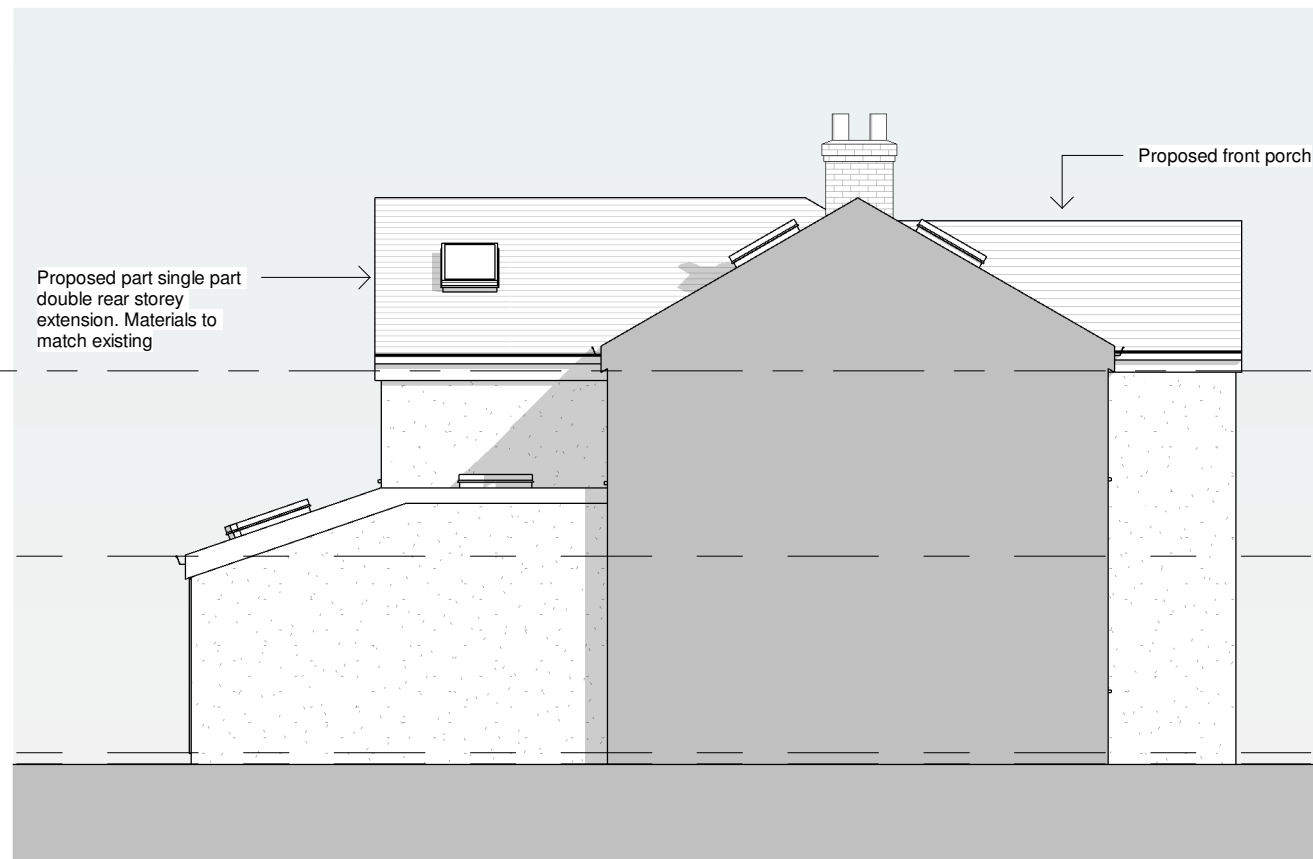
2 Proposed East Elevation 1 : 100
