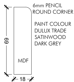
MDF DOOR AND SCREEN ARCHITRAVE SCALE 1:2
