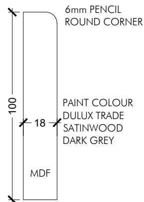
MDF TIMBER SKIRTING SCALE 1:2
