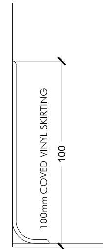
PVC FLOORING EDGE DETAIL WITH COVERED SKIRTING TYPE B - CLINICAL AREAS - GP SURGERY WAITING ROOM SCALE 1:2
