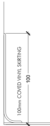
PVC FLOORING EDGE DETAIL WITH COVERED SKIRTING TYPE A - KITCHENS, TOILETS AND CLINICAL AREAS- TREATMENT AND THERAPY ROOMS SCALE 1:2
