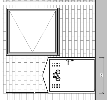
Cycle Storage - Side Elevation 1 : 20
