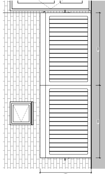
Cycle Storage - Front Elevation 1 : 20
