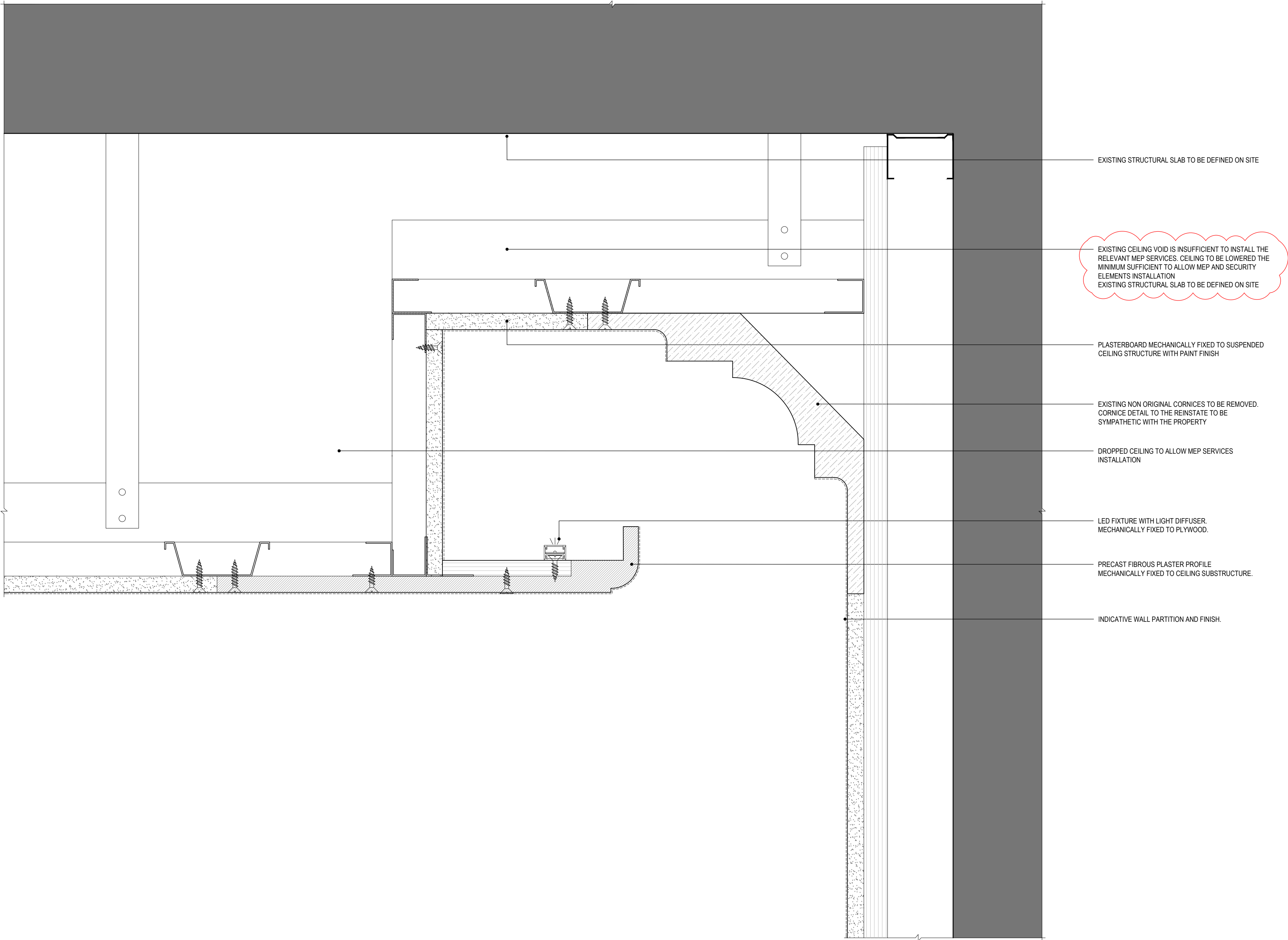
1 INDICATIVE CEILING DETAIL SCALE 1:2@A1
