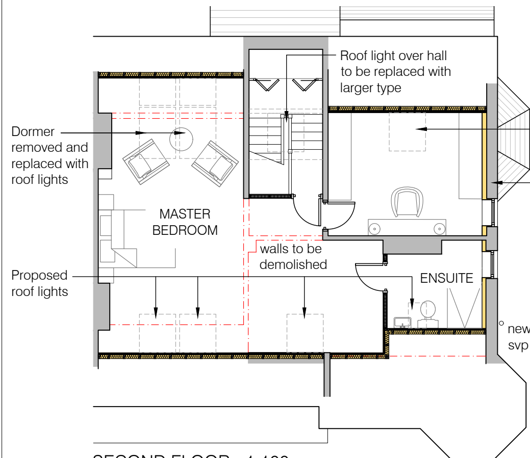
SECOND FLOOR - 1:100
