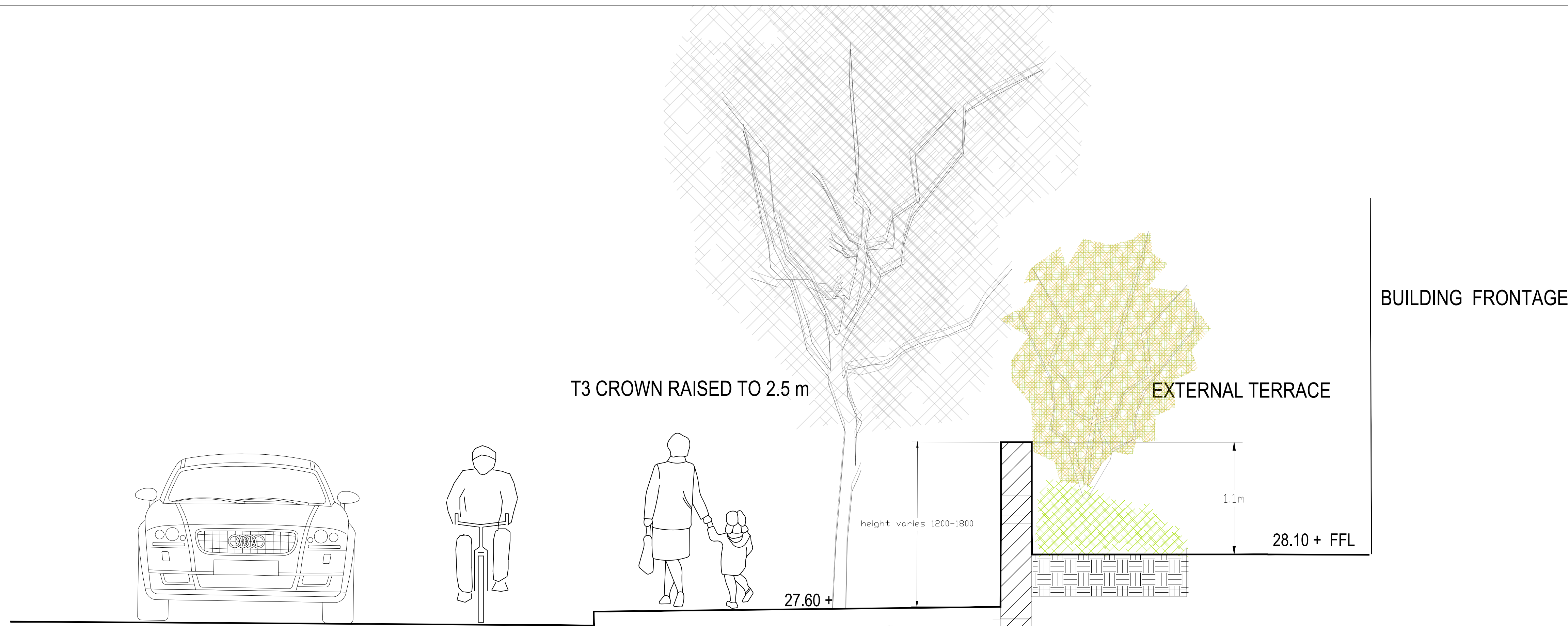
SECTION THROUGH MANCHESTER ROAD TO BUILDING FRONTAGE 1:25
