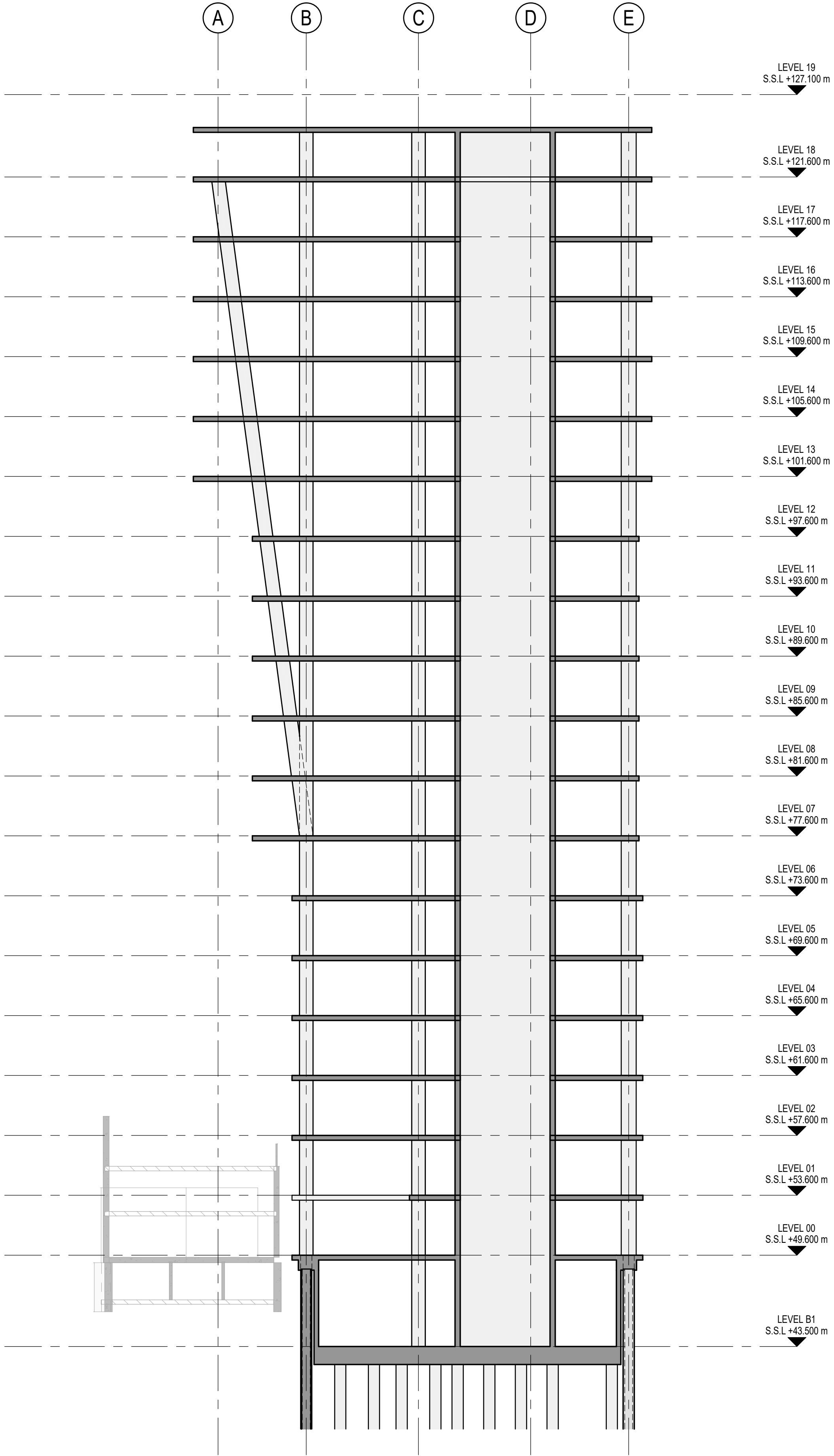
BUILDING SECTION 2 1 : 200
