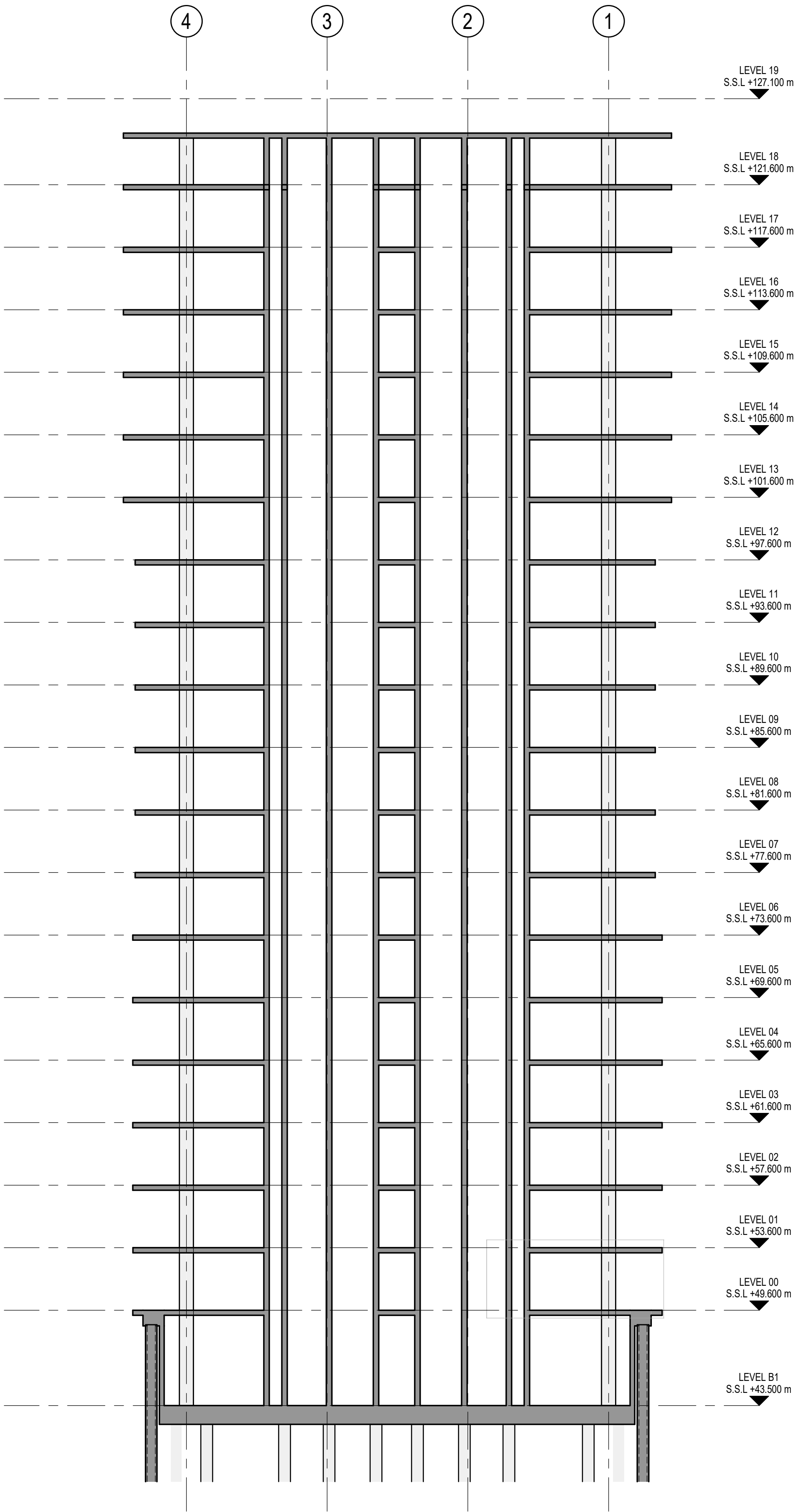
BUILDING SECTION 1 1 : 200
