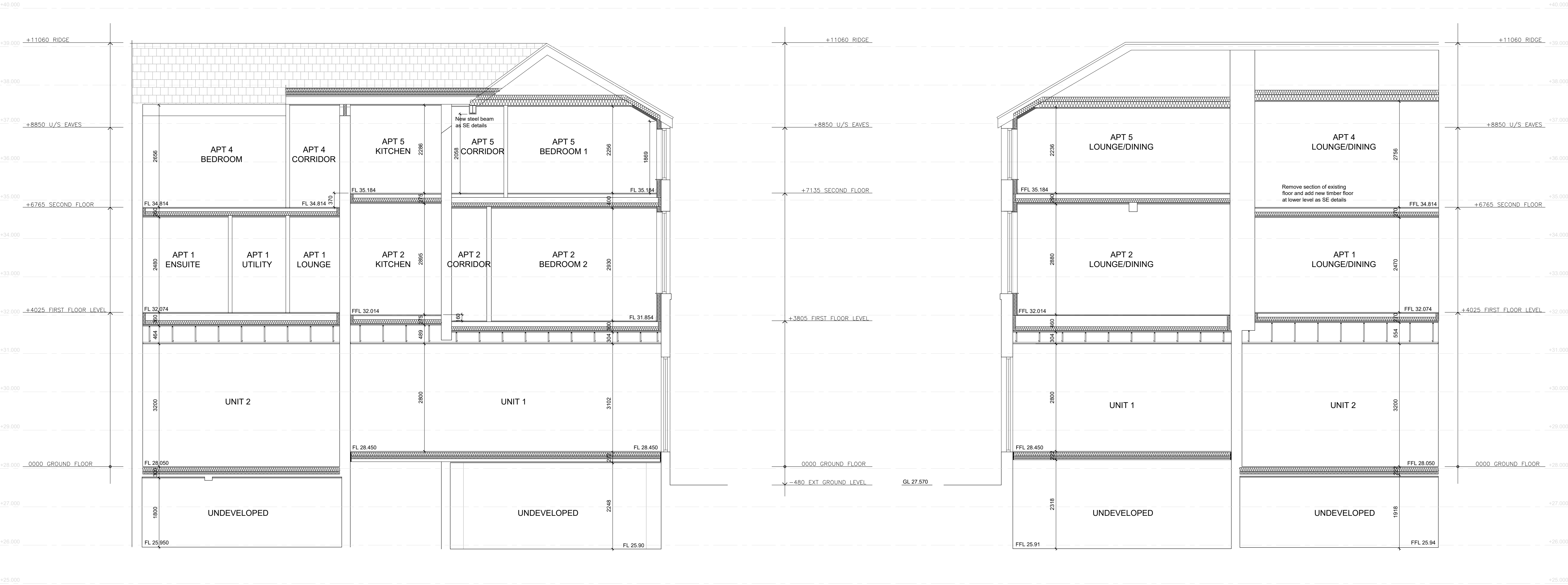
SECTION B-B
