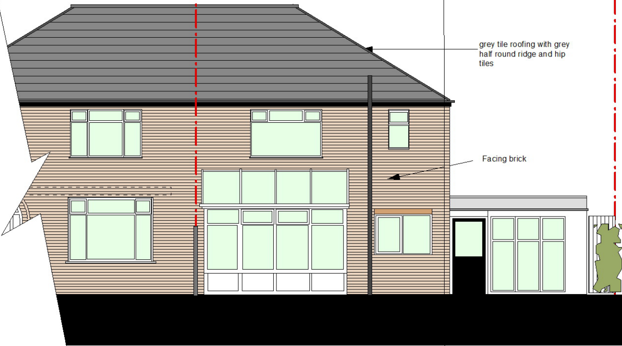
REAR ELEVATION AS EXISTING (EAST)
