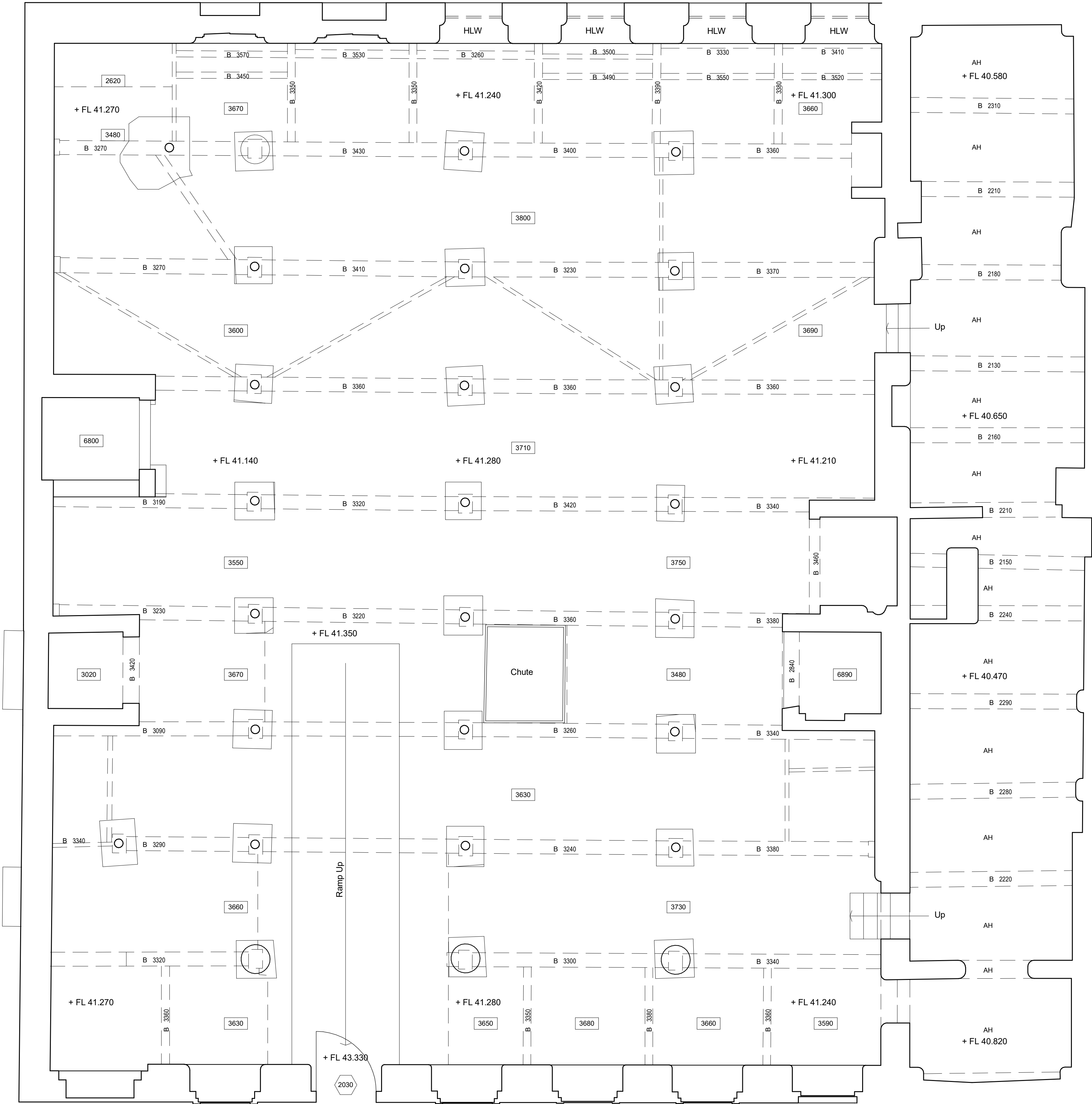
1 | Lower Ground floor - existing Copy 1
