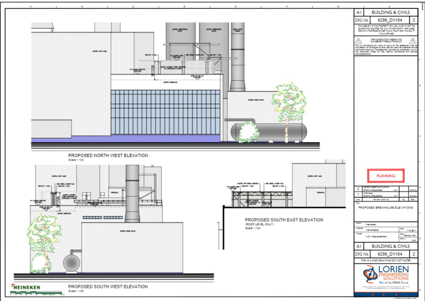
Figure 2. Proposed elevations
