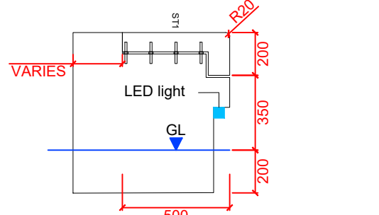
SPECIAL UNIT 21 INC TIMBER TOP DETAIL 019 SECTION @ 1:25
