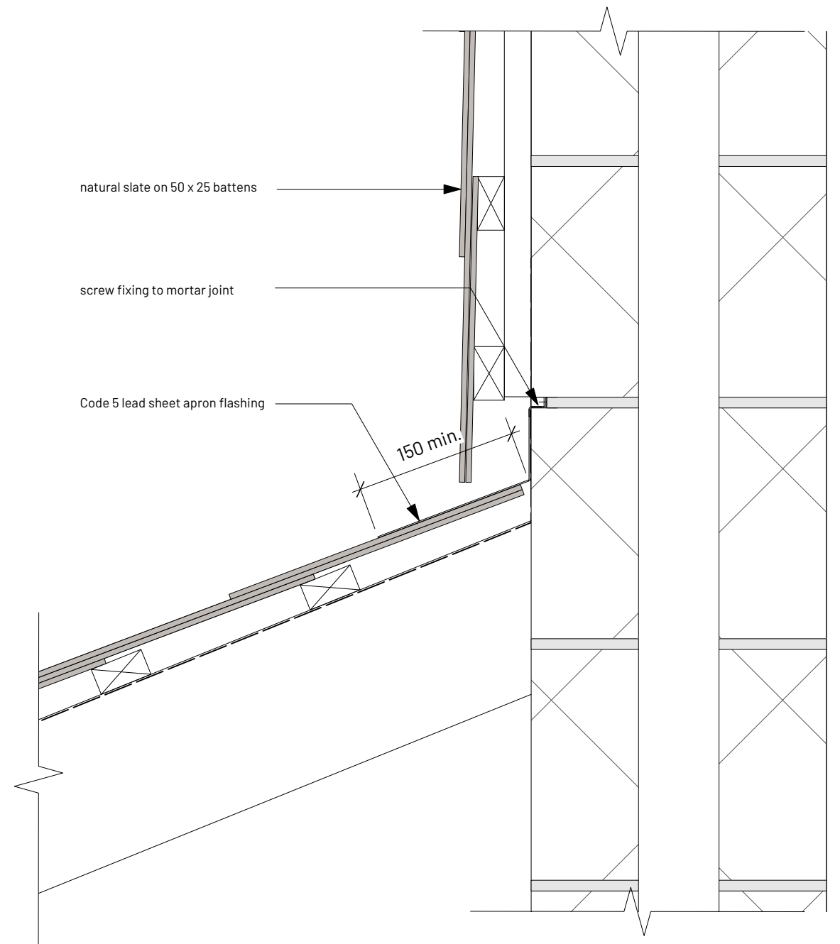
2 Top Edge Abutment Detail Scale: 1:5 See NBS Clause H71/410
