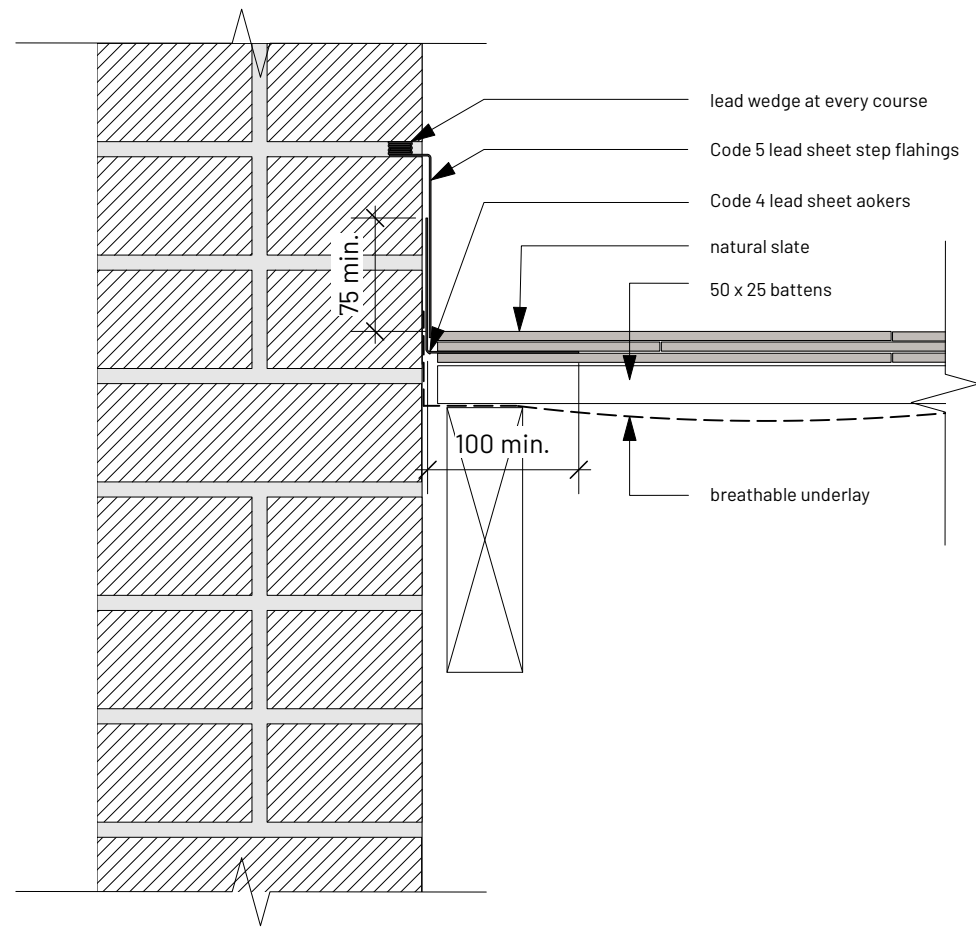
1 Roof Side Abutment Detail 1 Scale: 1:5 See NBS Clause H71/440
