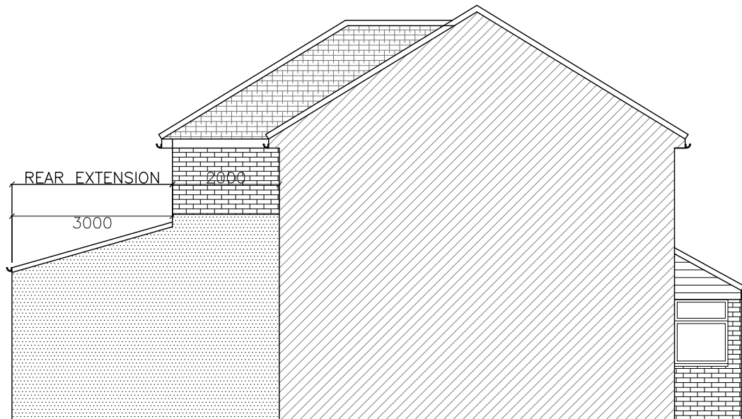
PROPOSED SIDE ELEVATION - B
