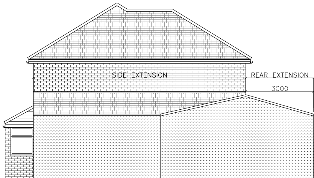
PROPOSED SIDE ELEVATION - A
