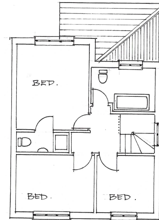
EXTG. FIRST FLOOR
