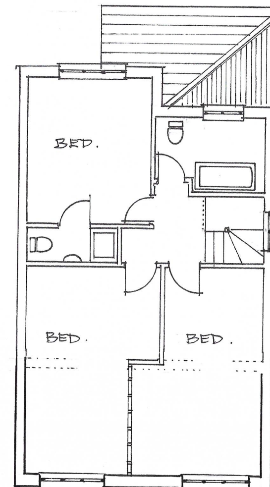
PROPOSED 1ST FLOOR
