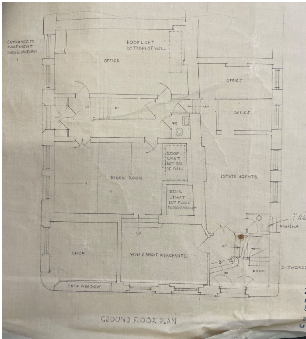
Figure 7: Clarence Street – Ground Floor Plan, c.1957. The plan of the building in the mid-20 th century is likely fairly similar to the original layout. A small shop was located to the north corner, apparently completely separate from the wider building, but may have previously have been connected. Directly adjacent to this a wine & spirit merchants is identified, with steps leading up into a stock room. Beyond this, a corridor with a central stair leading out onto 10 Kennedy Street can be seen, with a WC to the end of the corridor. The other areas of the building are shown to have been used for office space, with an estate agent to the Source: Manchester Archives.
