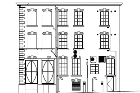
EXISTING NORTHEAST ELEVATION BOW LANE FACADE
