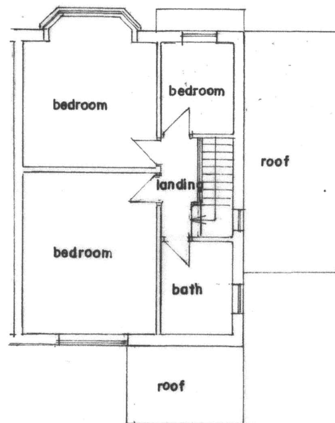
FIRST FLOOR PLAN (EXISTING)
