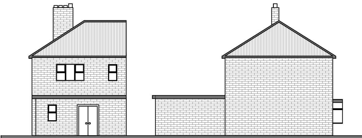
Proposed Rear Elevation Proposed Side North Elevation
