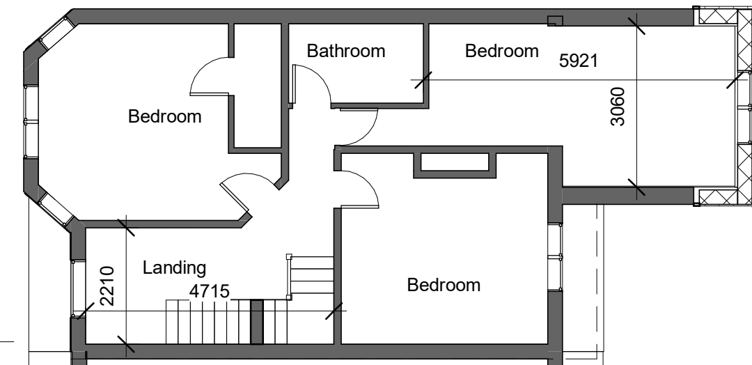
2 01 First Floor Proposed 1 : 100
