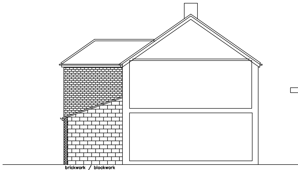
SIDE ELEVATION (facing No 29)Hidden by existing adjoining extension
