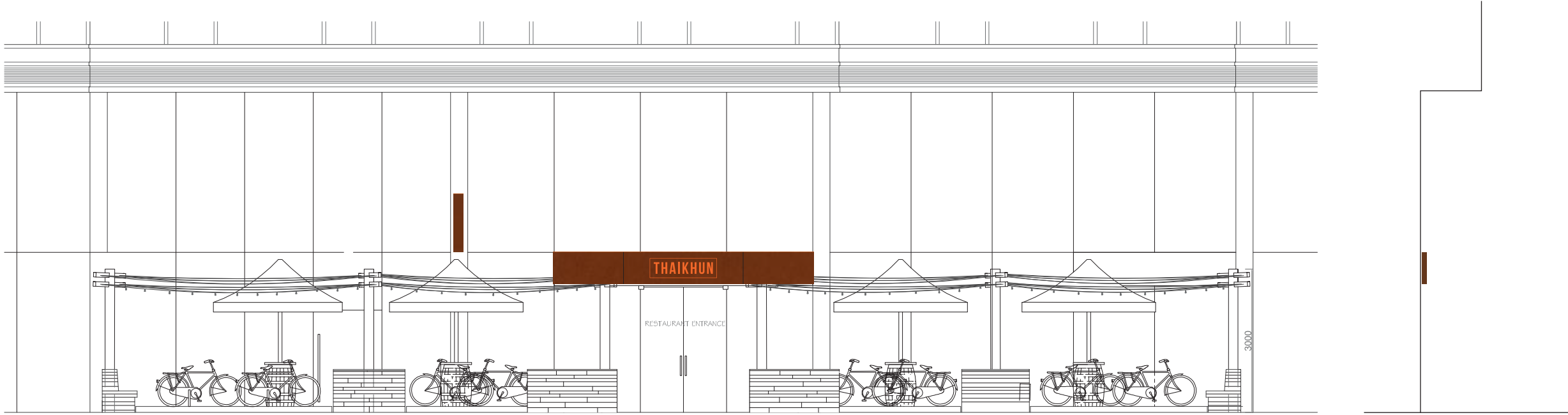
FRONTELEVATION- Scale 1:100@ A3
