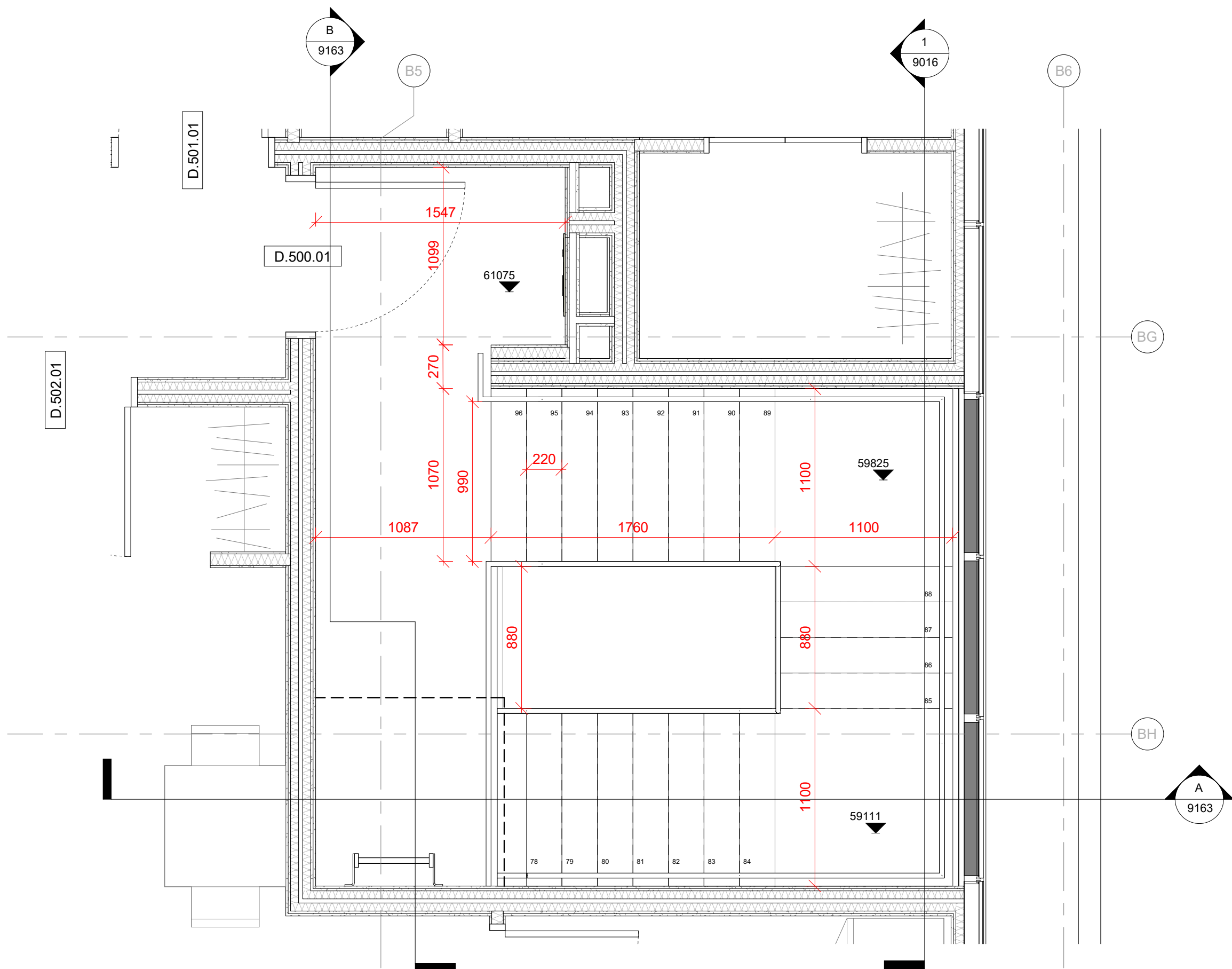
MAIN STAIRCASE - FIFTH FLOOR. 1 : 25
