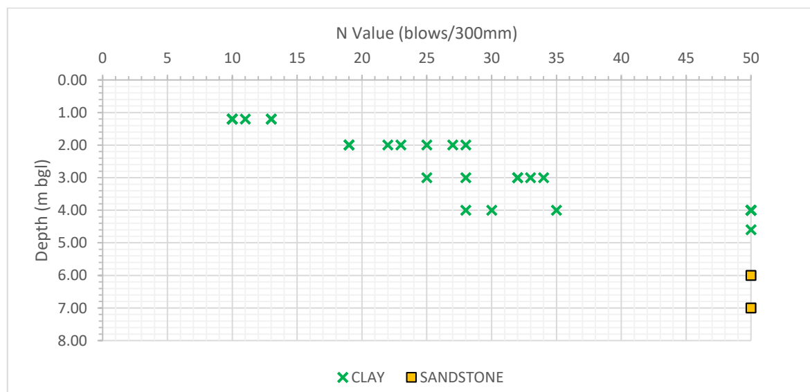
Figure 4: SPT Results
