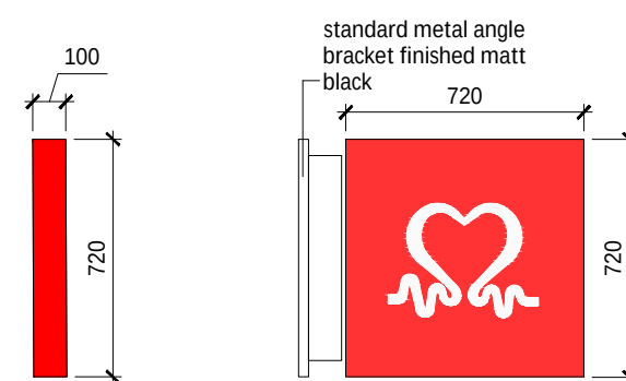
Sign 2: Projector Sign Detail (Scale 1/25) Illuminated
