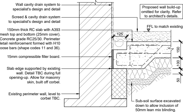
Figure 22 Proposed concrete slab detail at perimeter walls [Source: Booth King] 17
