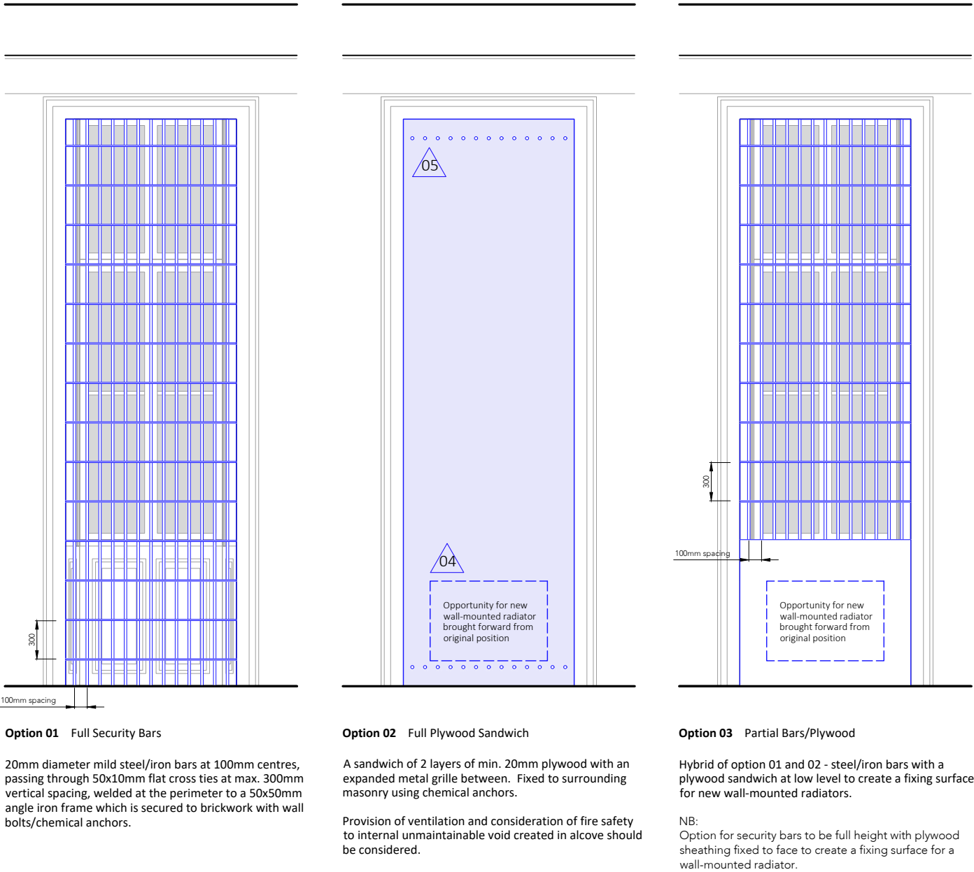
Figure 34 Alternative discounted window security options
