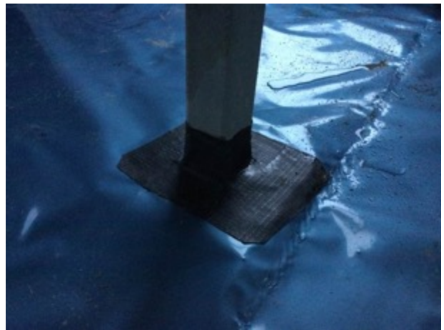
Steel column detailing sealed with SAGM to Unit D office area.
