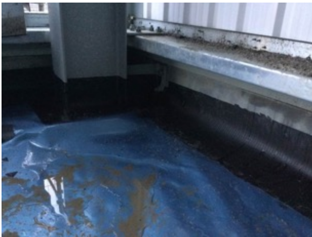
Retro detailing and steel stanchion detailing sealed with SAGM.
