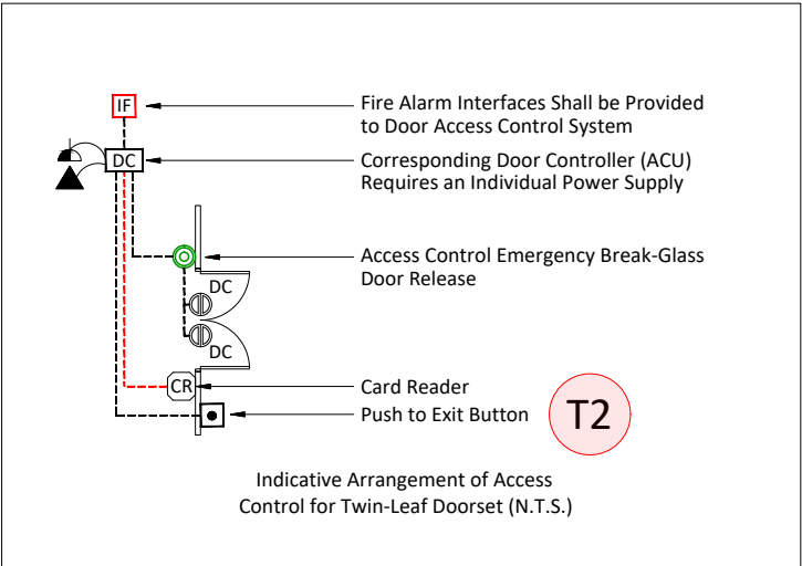
Indicative Arrangement of Access Control for Twin-Leaf Doorset (N.T.S)
