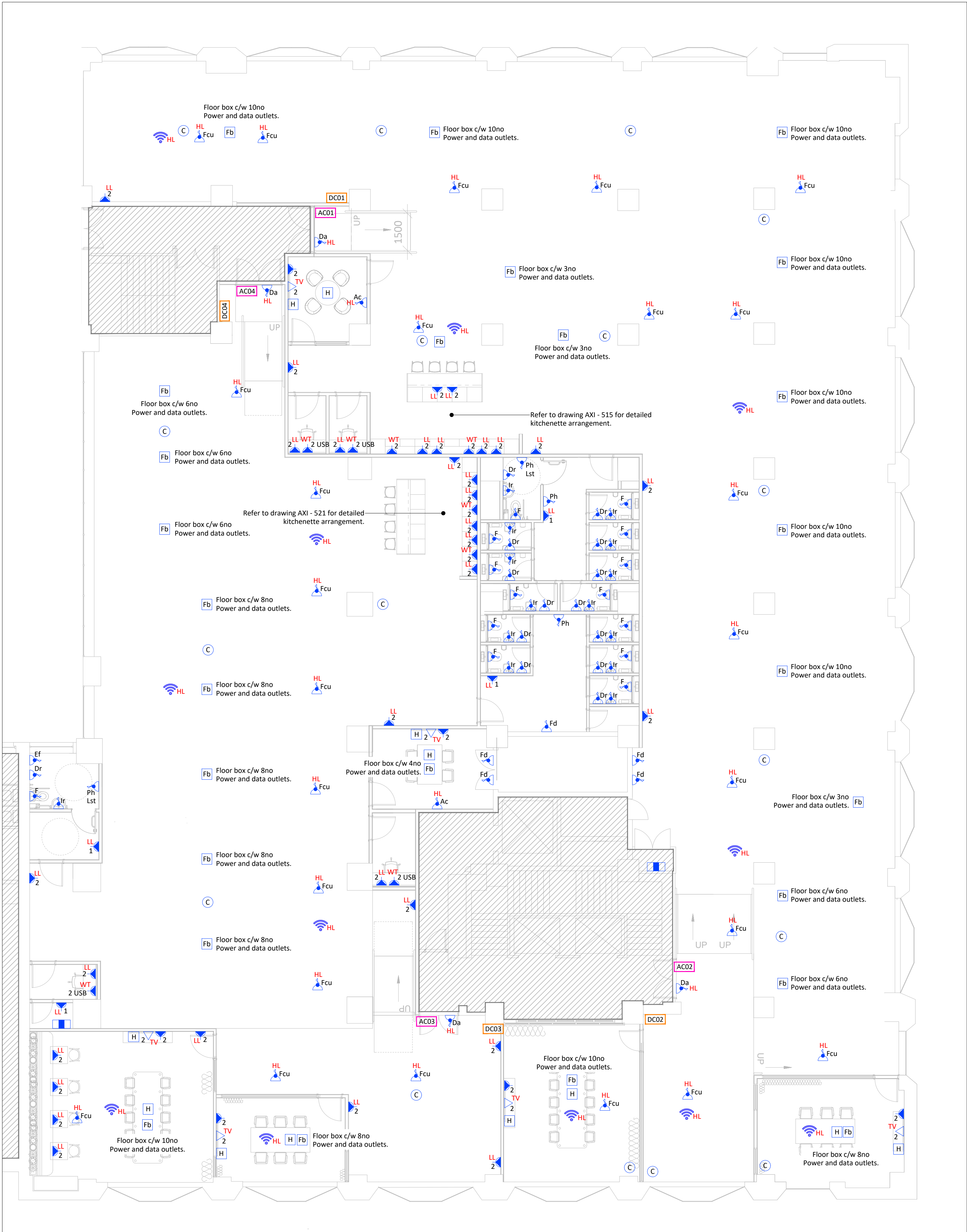
Lee House | Third Floor Small Power, Data & Security
