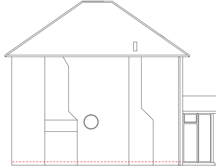
WEST SIDE ELEVATION
