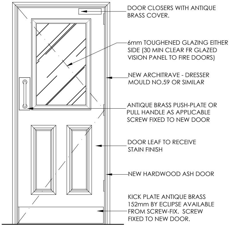
DOOR TYPE C - GENERAL INTERNAL CIRCULATION DOORS
