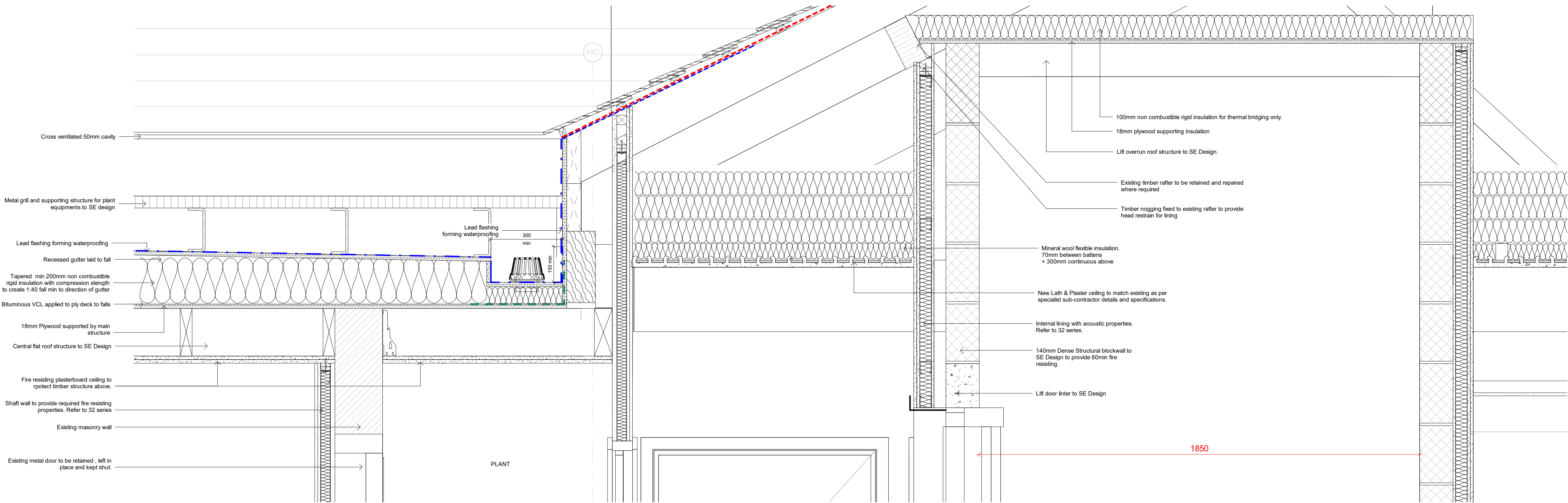
1 | Roof details - Central deck + lift overrun. SCALE 1 : 10 @A1
