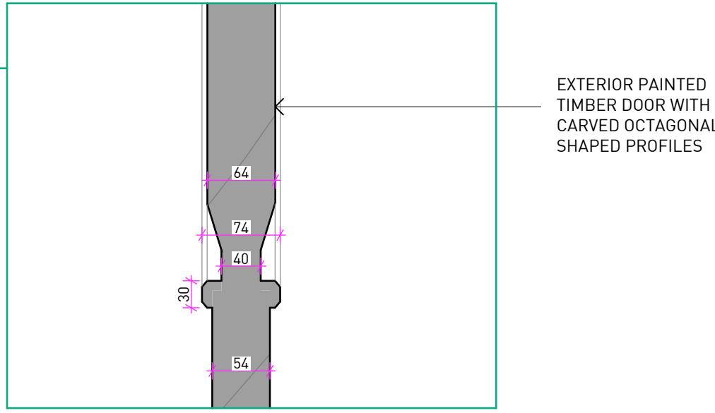
DETAIL 03 - 1:5
