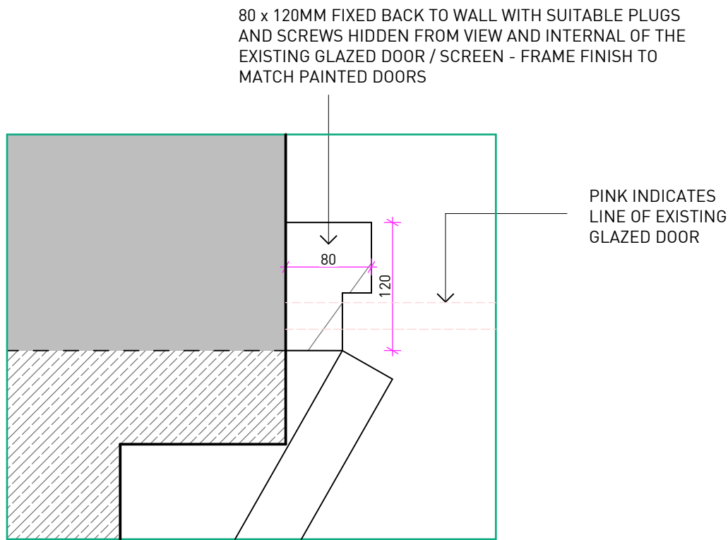
DETAIL 01 - 1:5
