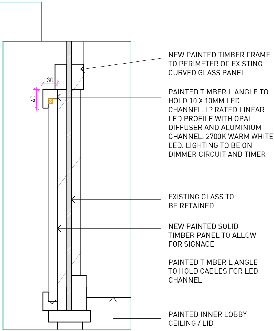
DETAIL 02 - 1:5
