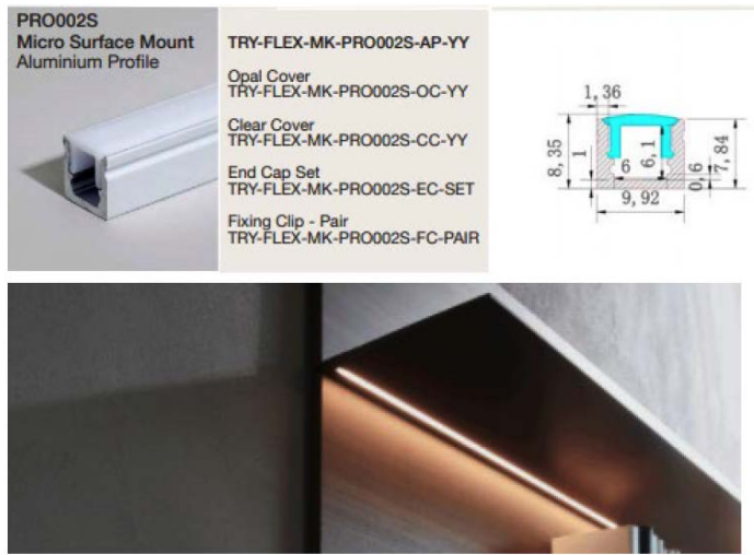
LED DETAIL SPEC: TRYKER - ADDER 180 IP LED SURFACE
