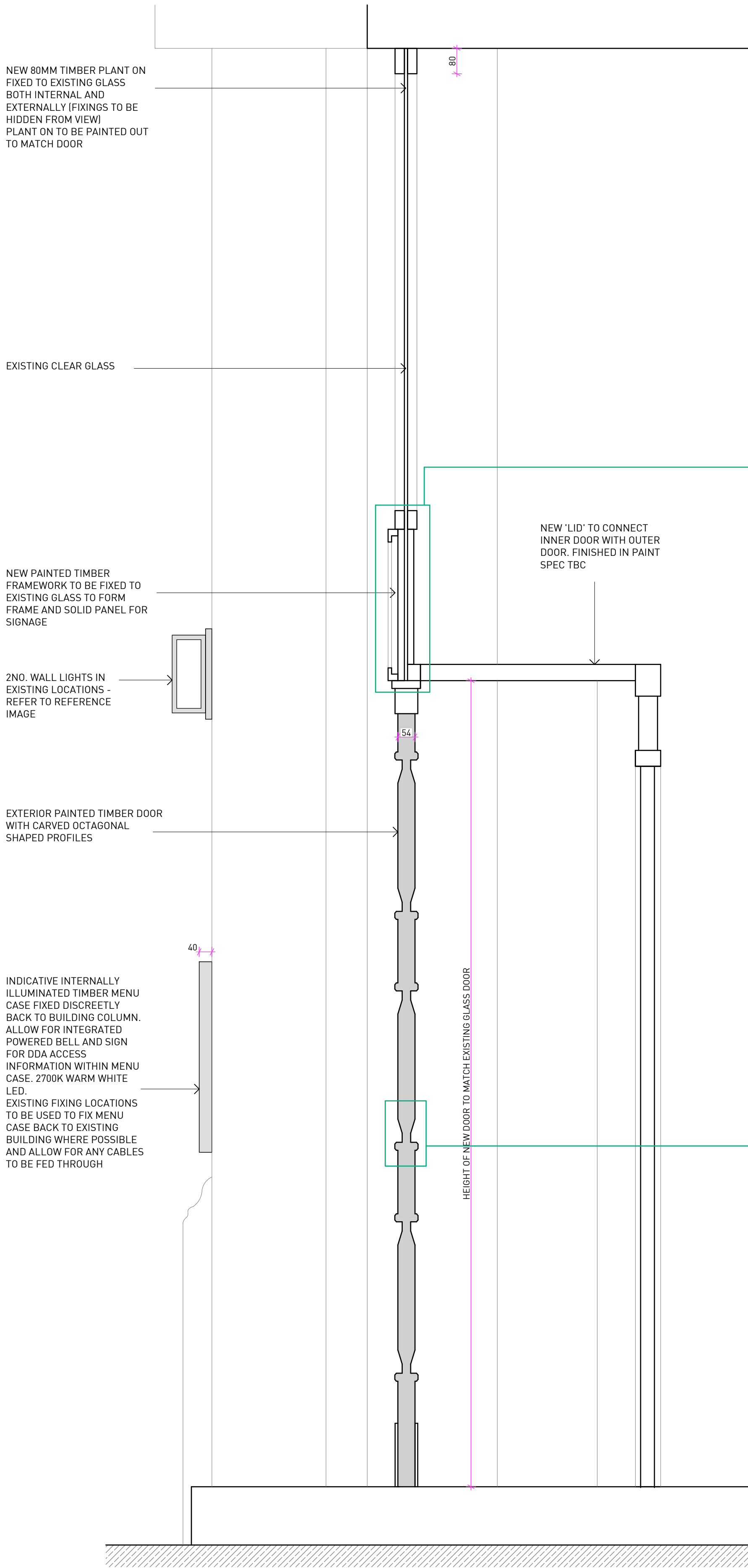
PROPOSED SECTION THROUGH ENTRANCE DOOR - 1:10
