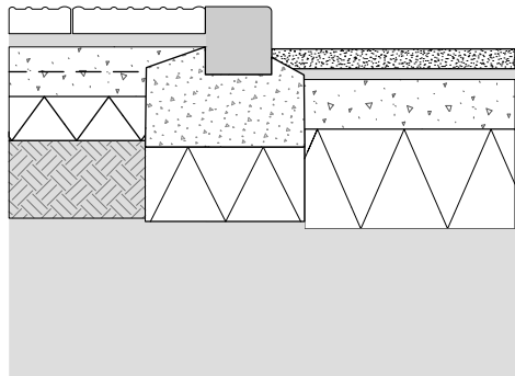
2 E2 Concrete Road Kerb Scale: 1:25
