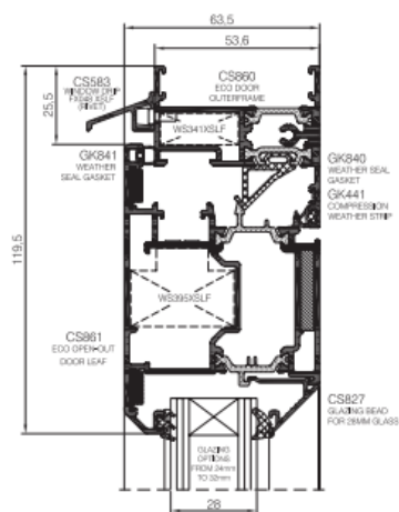
Comar 7P.i. ECO Door 55mm, Open-out
