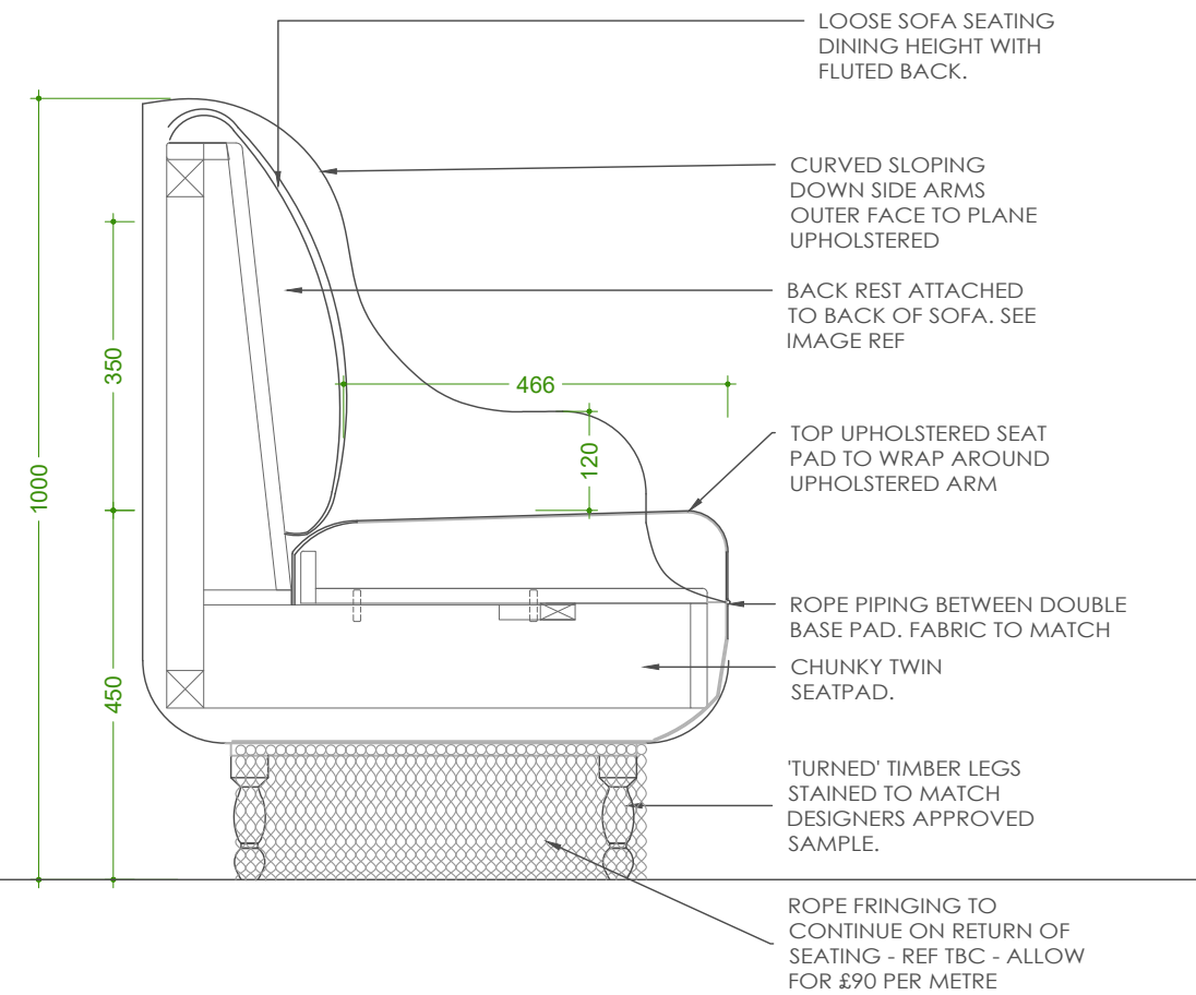
SOFA STYLE FIXED SEATING - SECTION THRU' Scale 1:20
