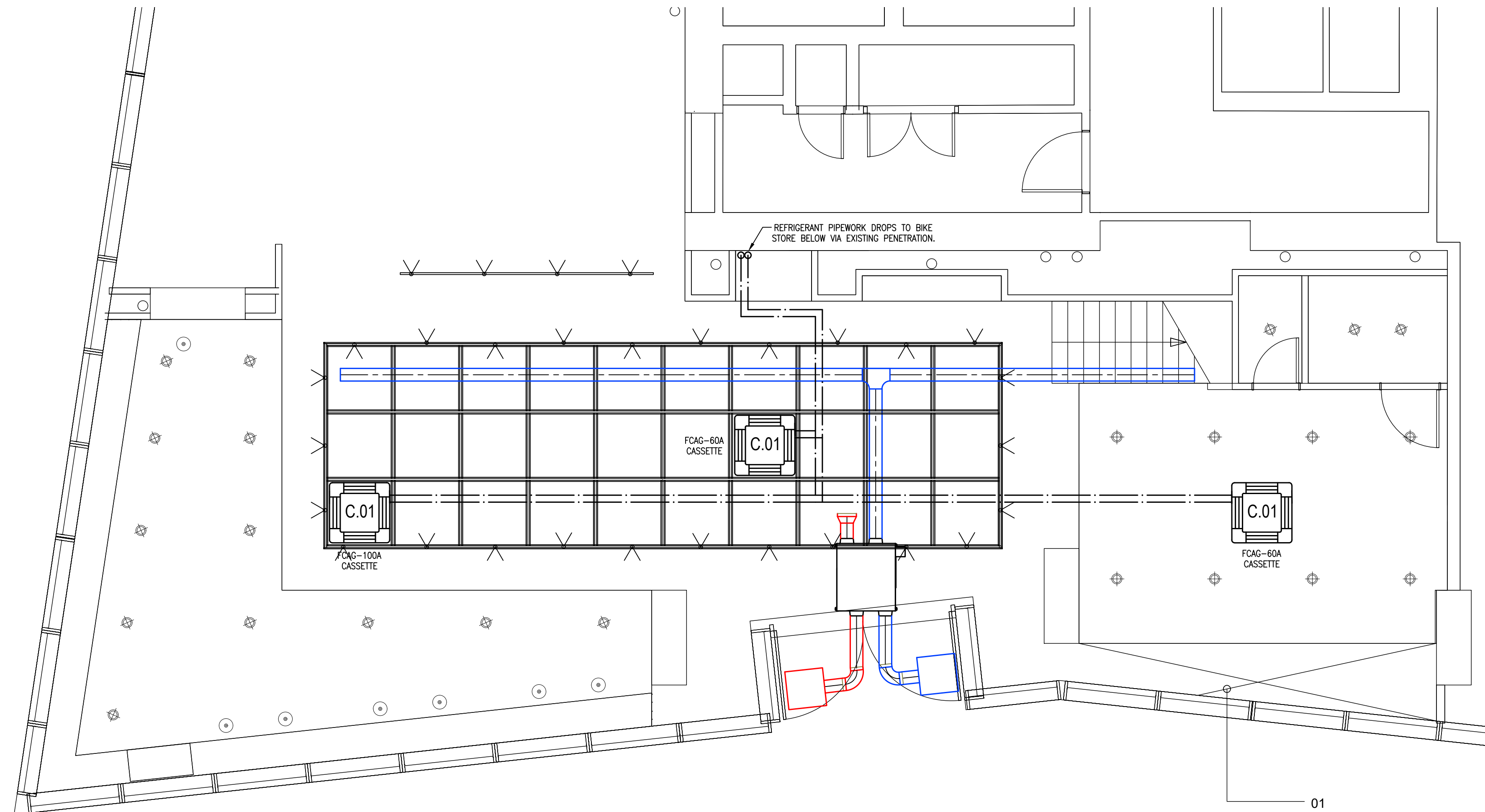
GROUND FLOOR - UNIT 7 SCALE 1:50
