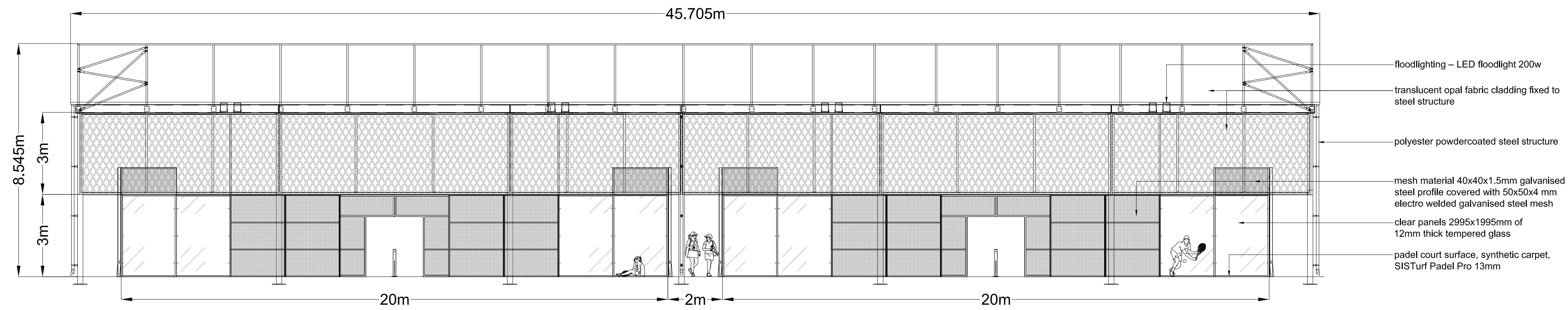
ELEVATION C (EAST)
