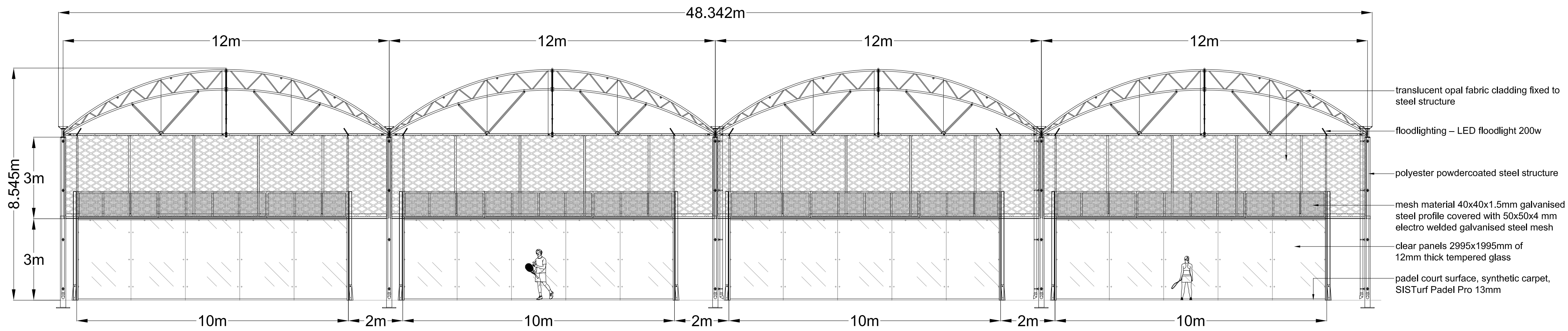
ELEVATION D (NORTH)
