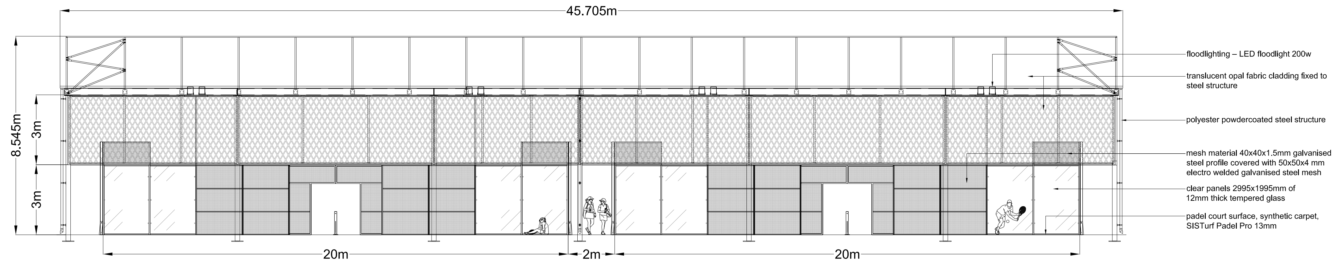
ELEVATION A (WEST)
