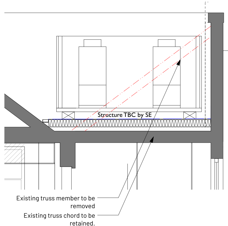
2 Plant Deck Section Scale: 1:50
