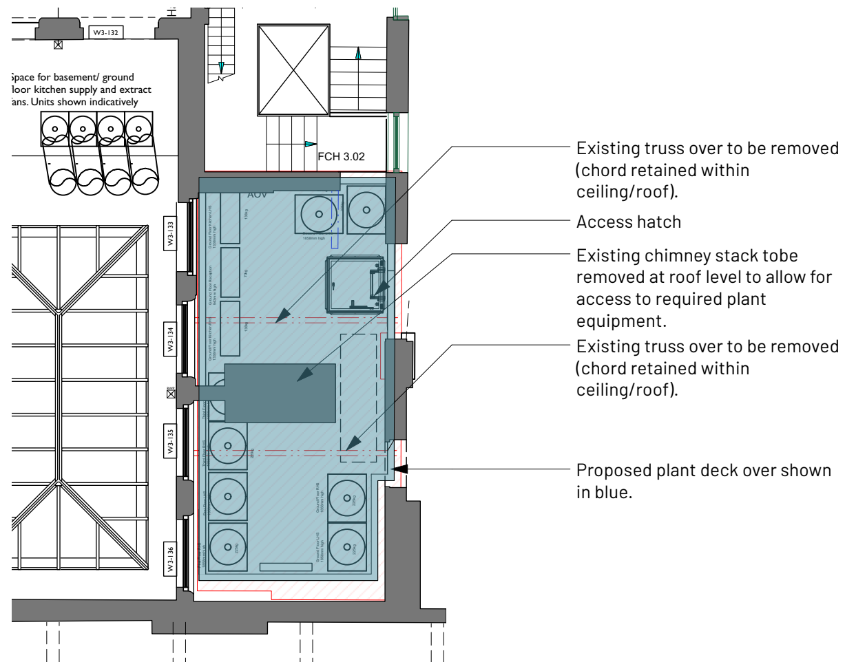
1 Proposed Reflected Ceiling and Plant Plan Scale: 1:100
