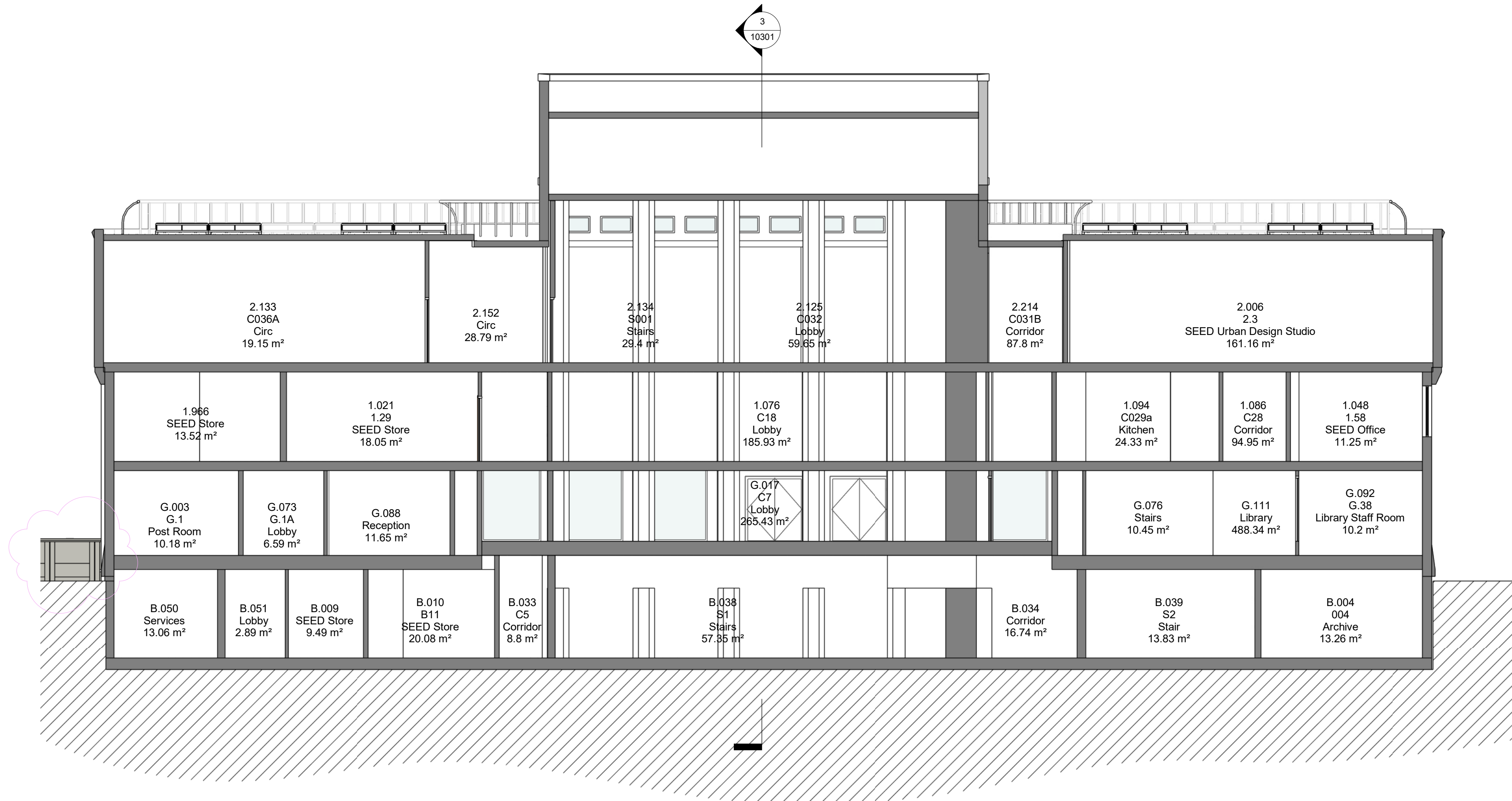
Short Section as Proposed
