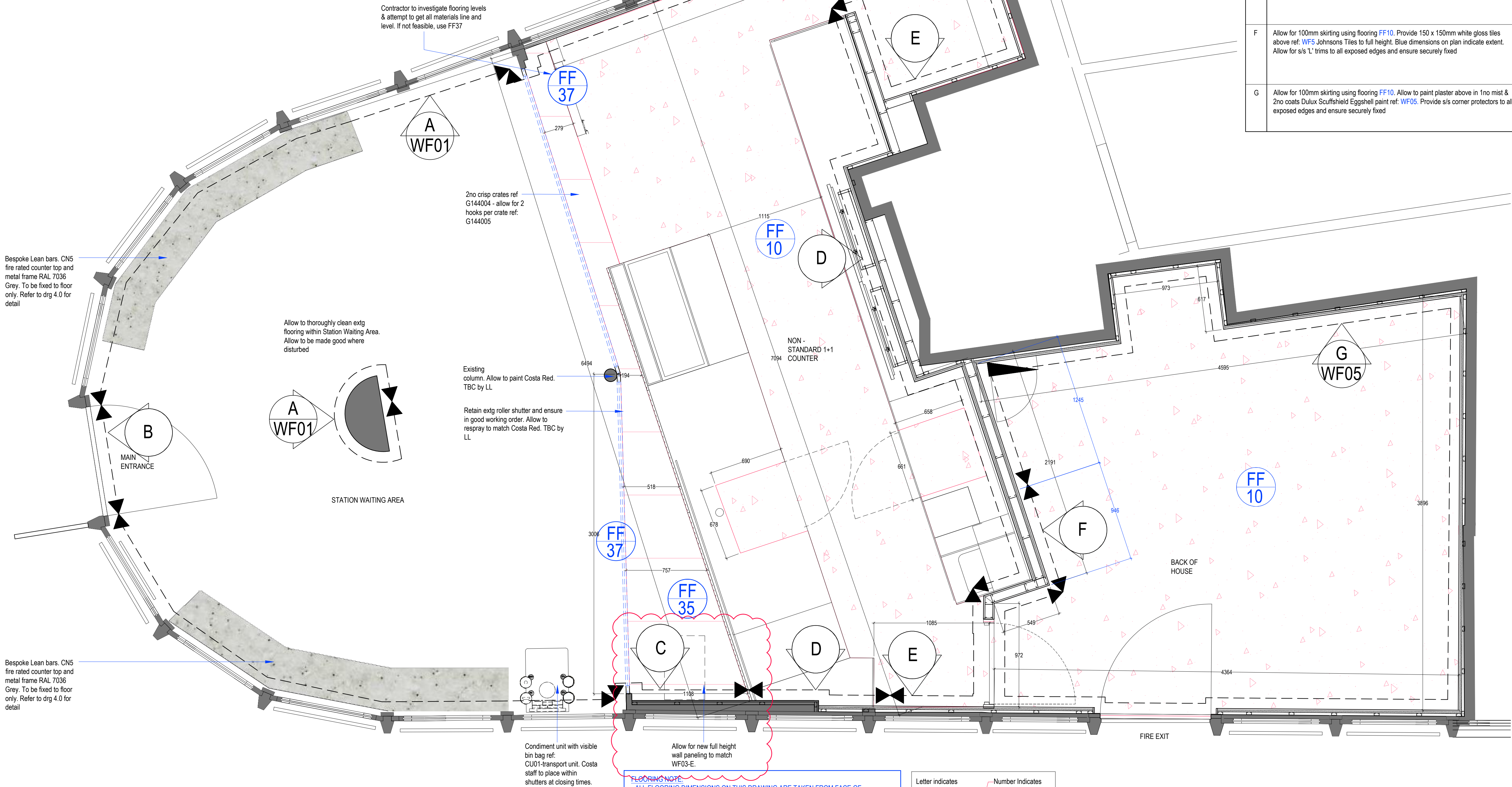
Proposed General Layout - SCALE 1:20
