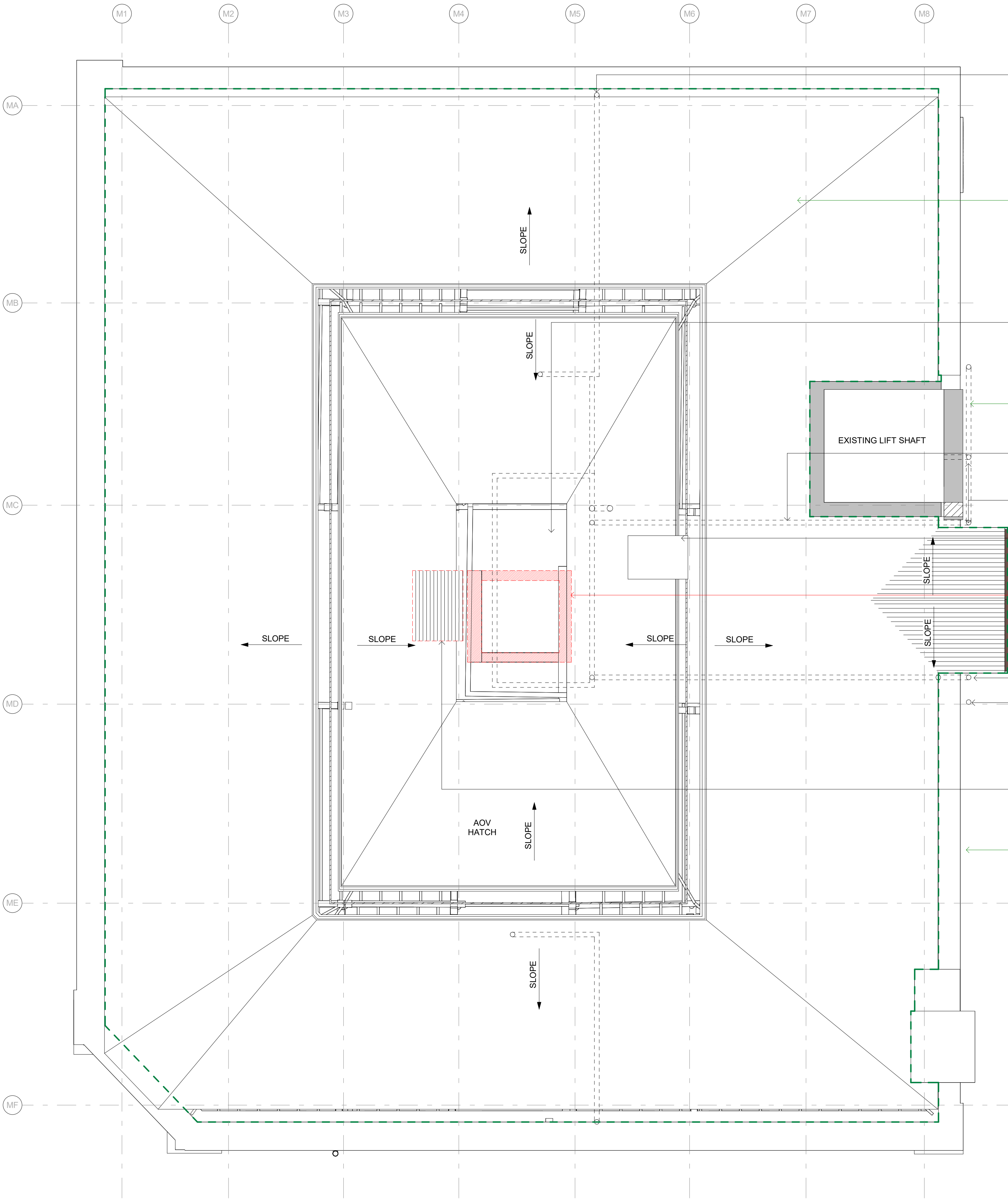
1 | MH - RP - Roof_Retention Plan. 1 : 50
