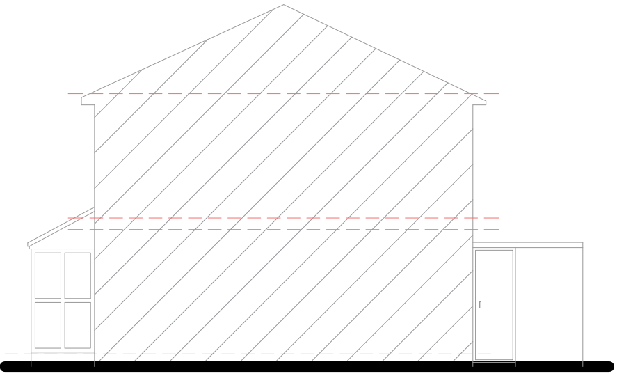
Side Elevation 2
