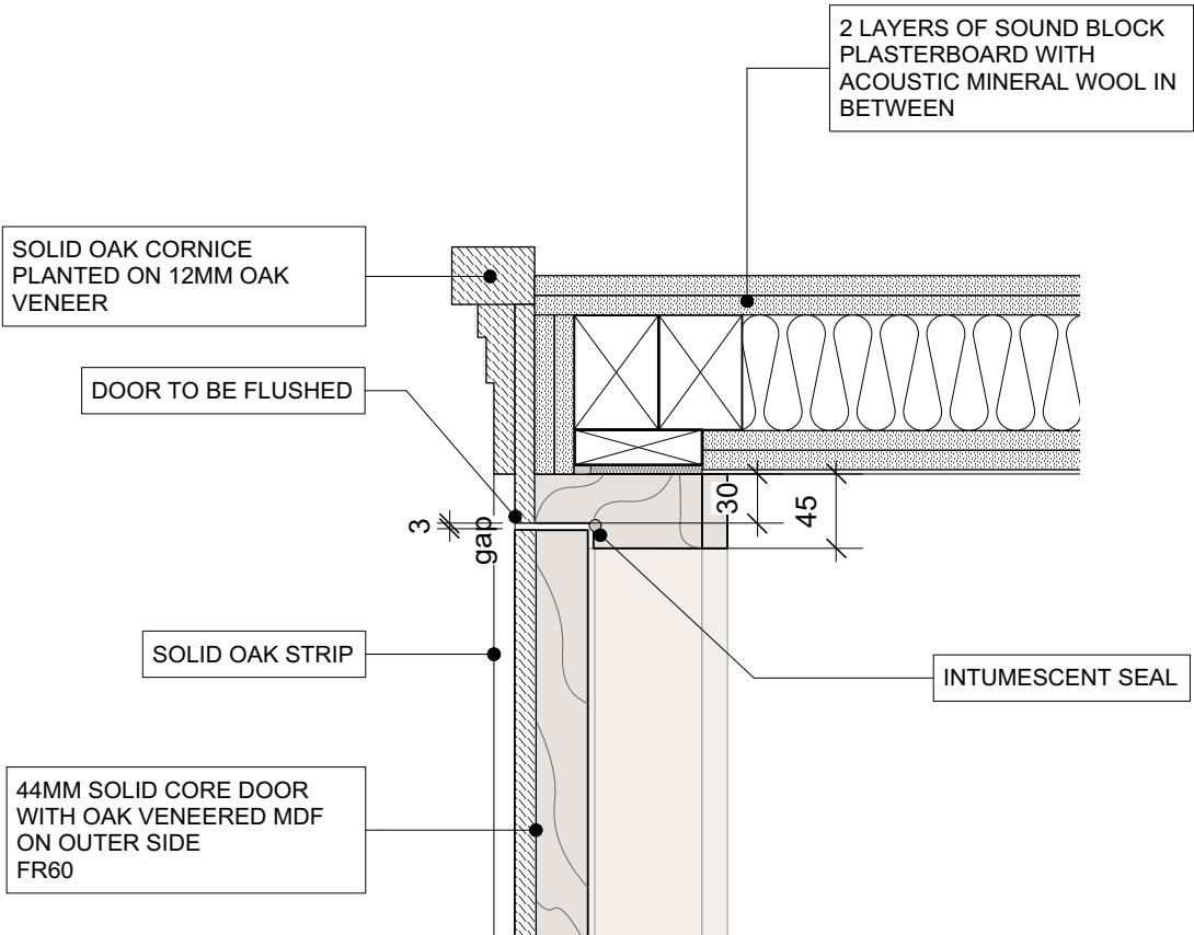
DETAIL 1
