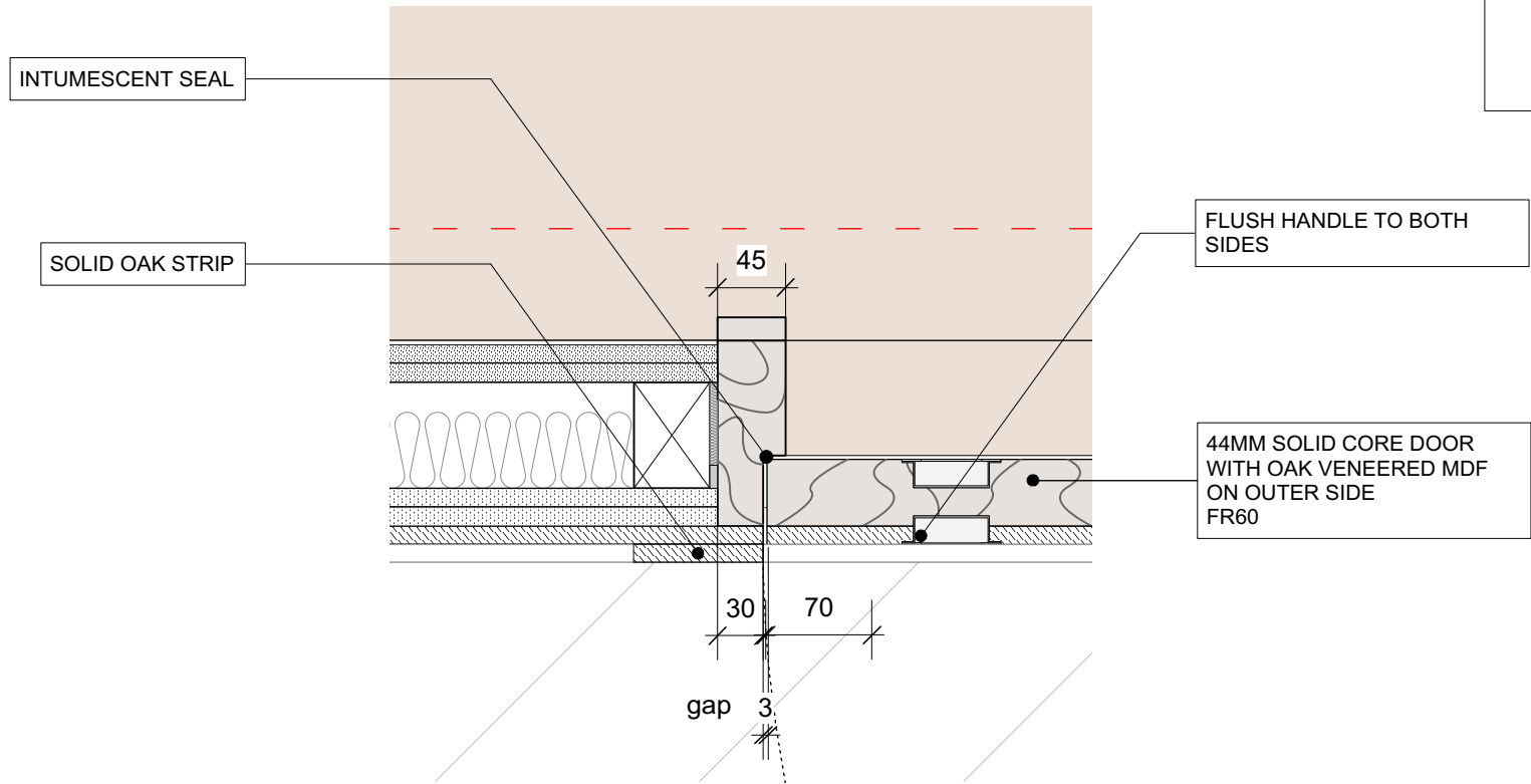
DETAIL 3
