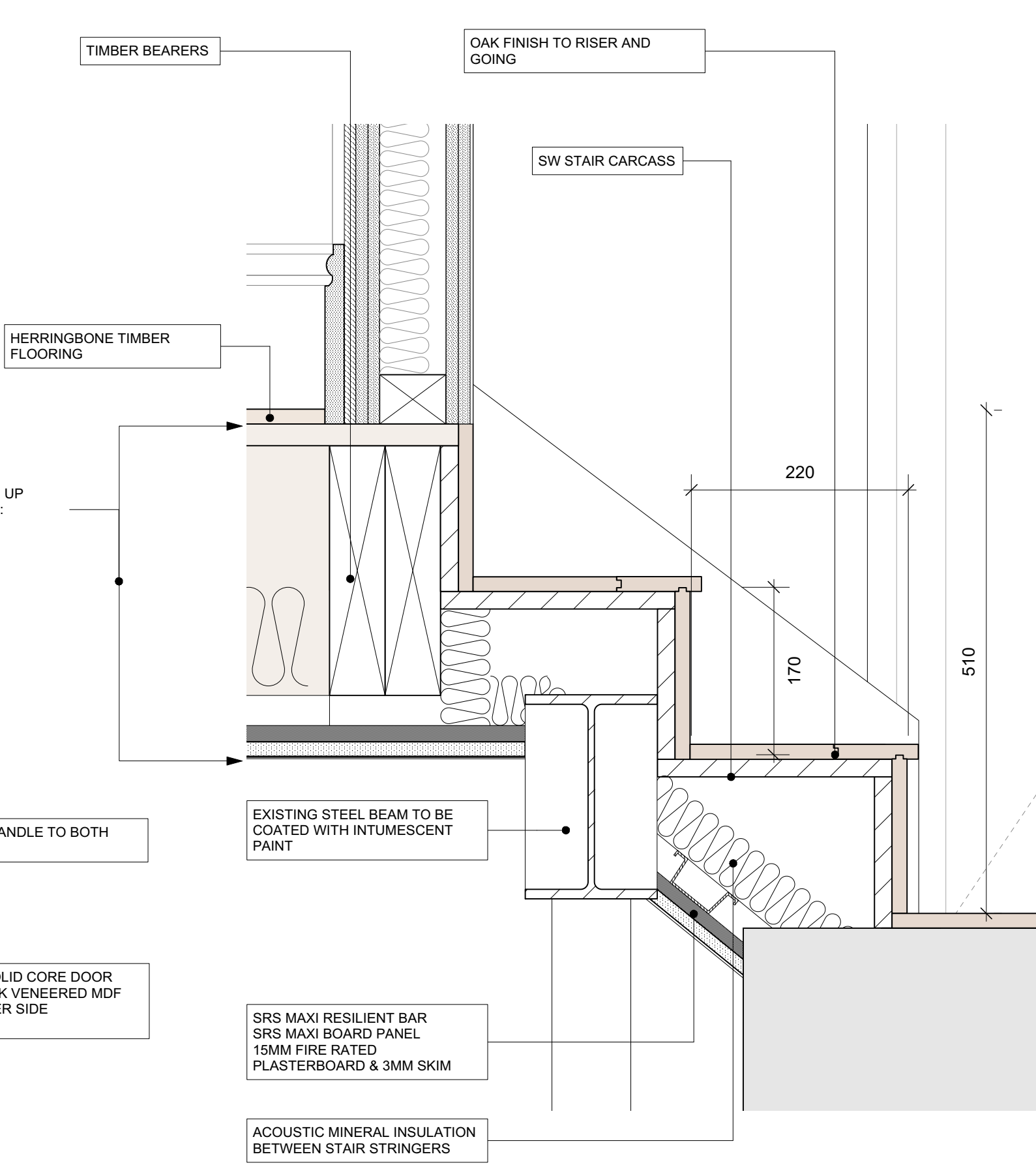
DETAIL 2
