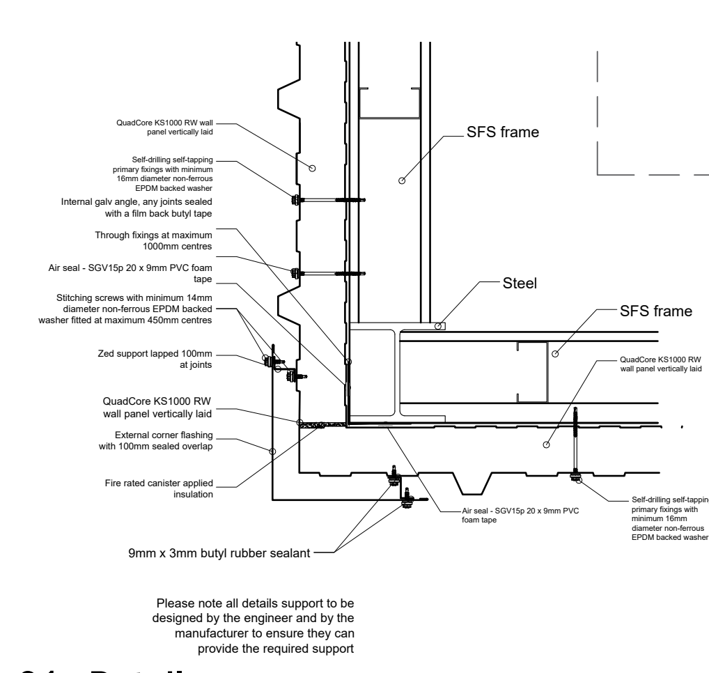
01 - Detail
