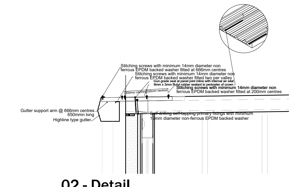
02 - Detail
