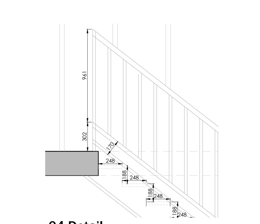
04 Detail
