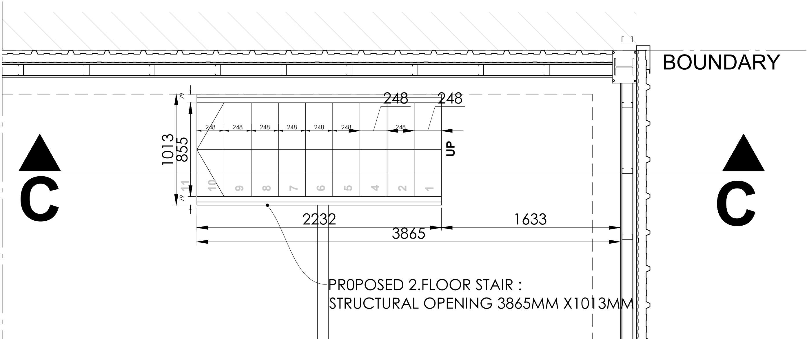
PROPOSED SECOND FLOOR STAIR PLANING DETAIL
