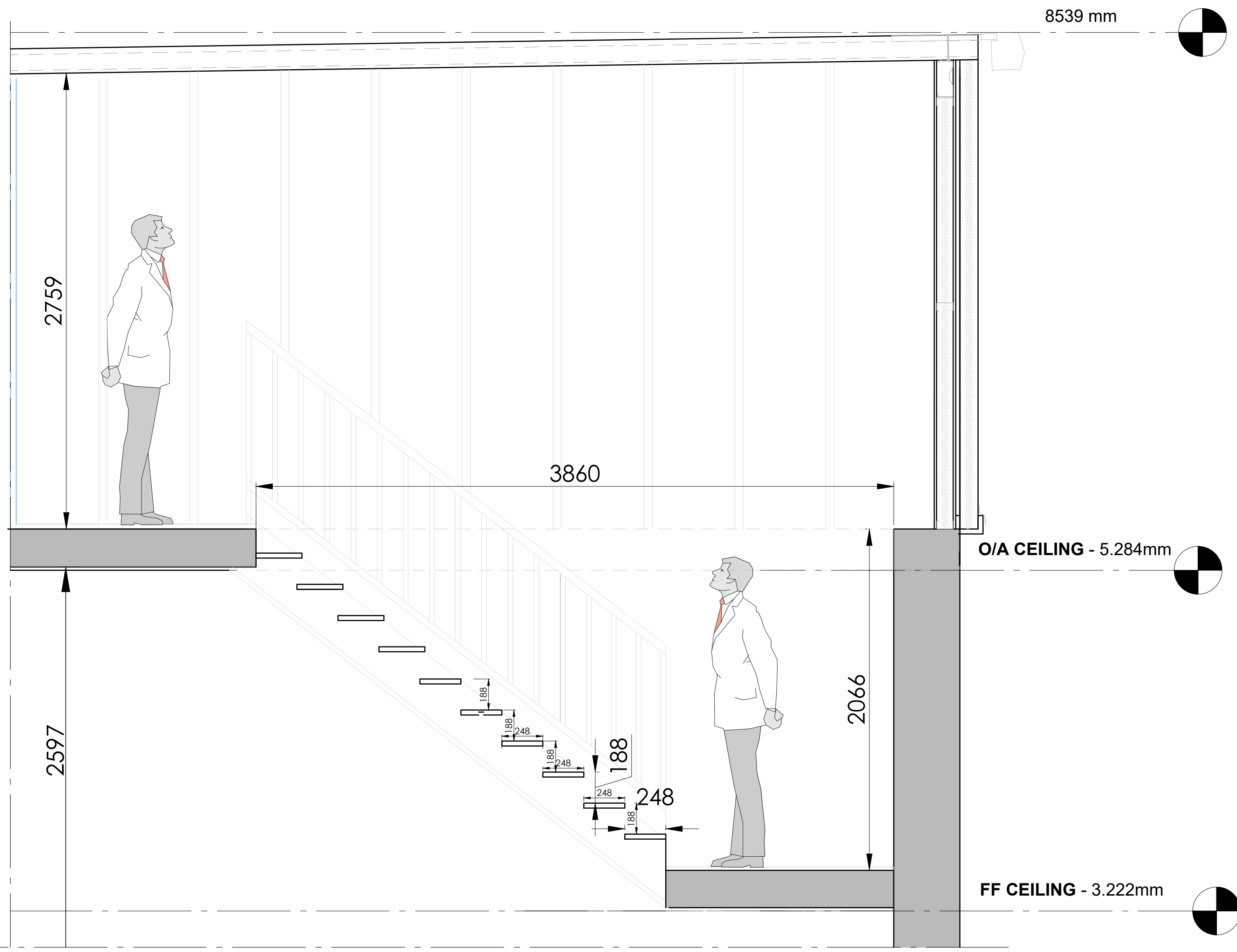
PROPOSED SECOND FLOOR STAIR PLANING DETAIL
