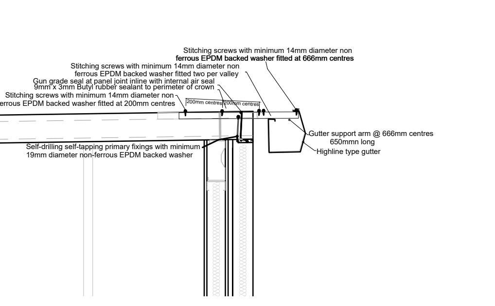
03 Detail
