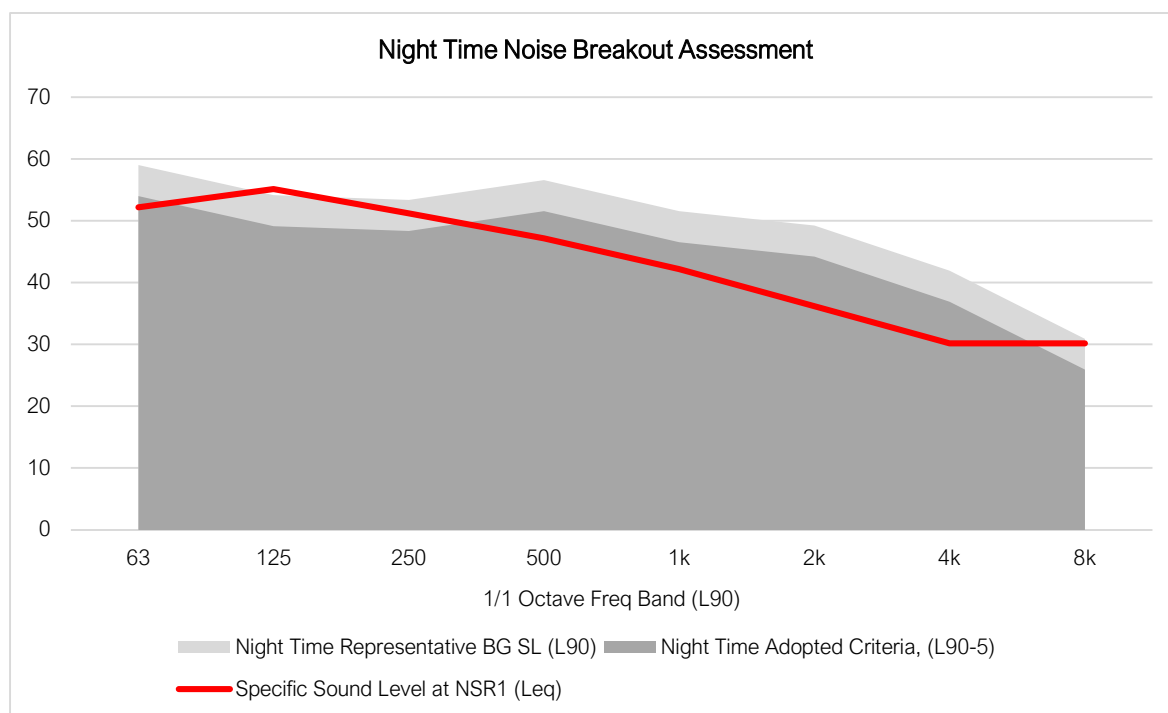
Figure 3 – Noise Breakout Assessment
