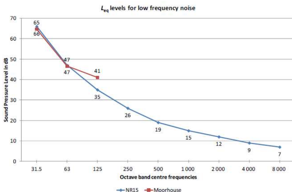
Figure 5 – Moorhouse Low Frequency Noise Rating Curve
